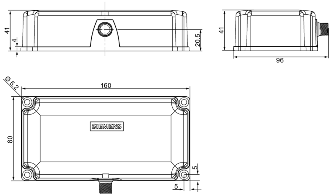
Figure 5-37 Dimension drawing
