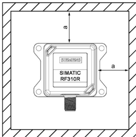
Figure 5-9 Metal-free area for RF310R
