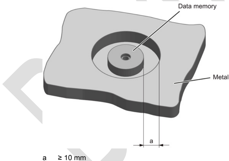
Figure 7-6 Mounting of the RF330T in metal with 10 mm clearance
