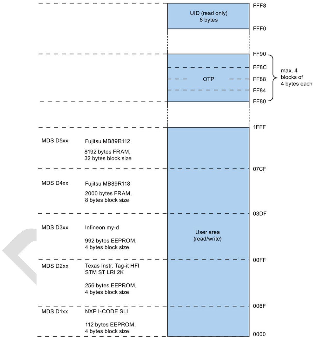
Figure 8-1 Memory configuration of ISO the transponders
