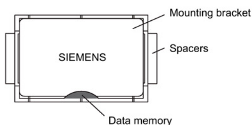
Transponder with mounting bracket and spacer (assembled)
