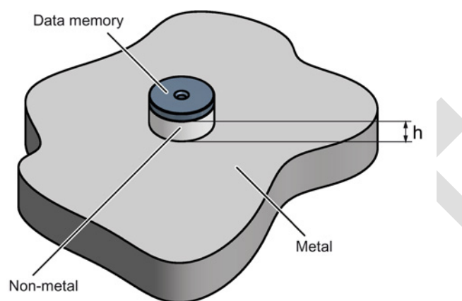
Figure 8-6 Mounting the MDS D124/D324/D424/D524/E624 and RF320T on metal with spacer
