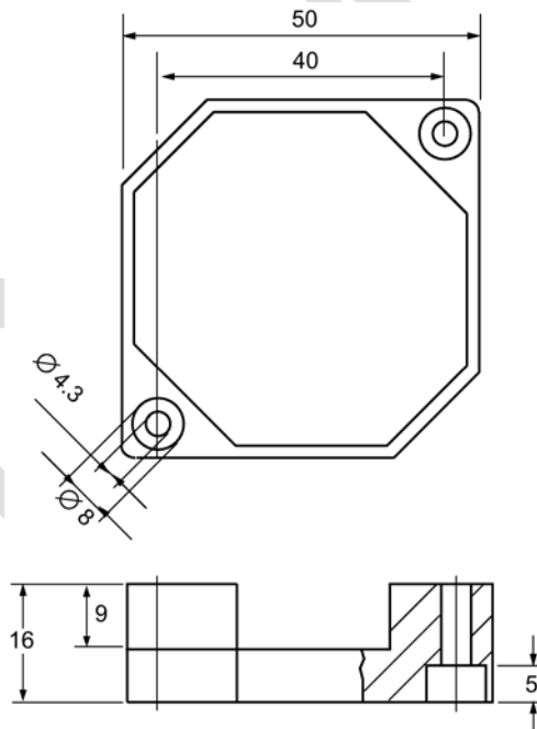
Figure 7-15 RF350T fixing frame
