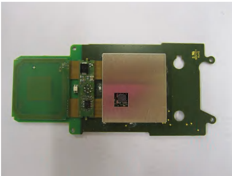
Picture 4. MOD board bottom with a shield.
