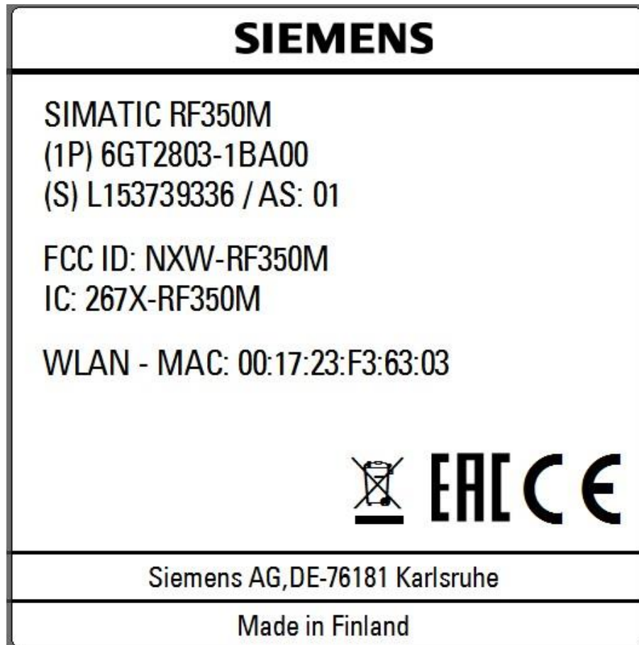
Picture 1. Simatic RF350M label.
