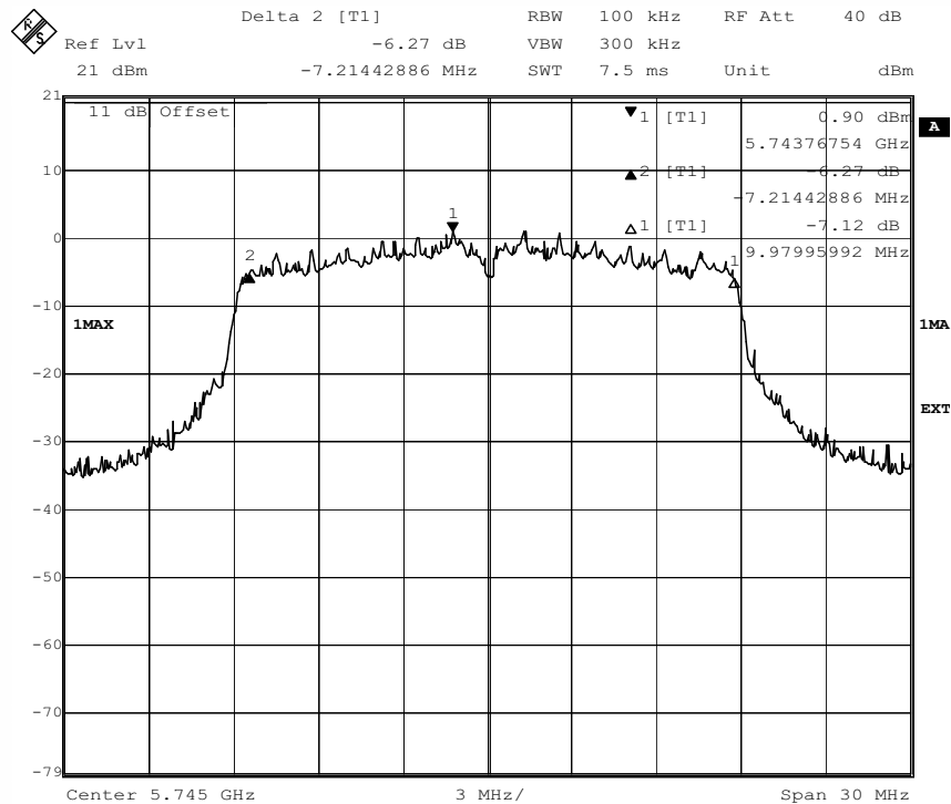
Screenshot: Occupied 6 dB bandwidth Measurement, channel 149
