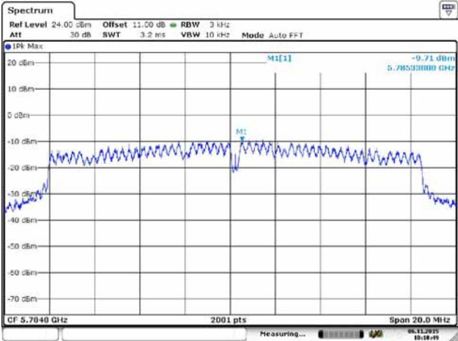
Screenshot: Average Output power, channel 157
