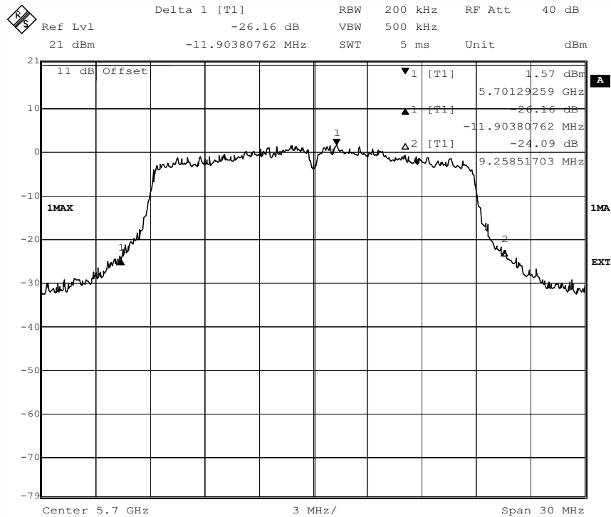
Screenshot: Occupied 26 dB bandwidth Measurement, channel 140
