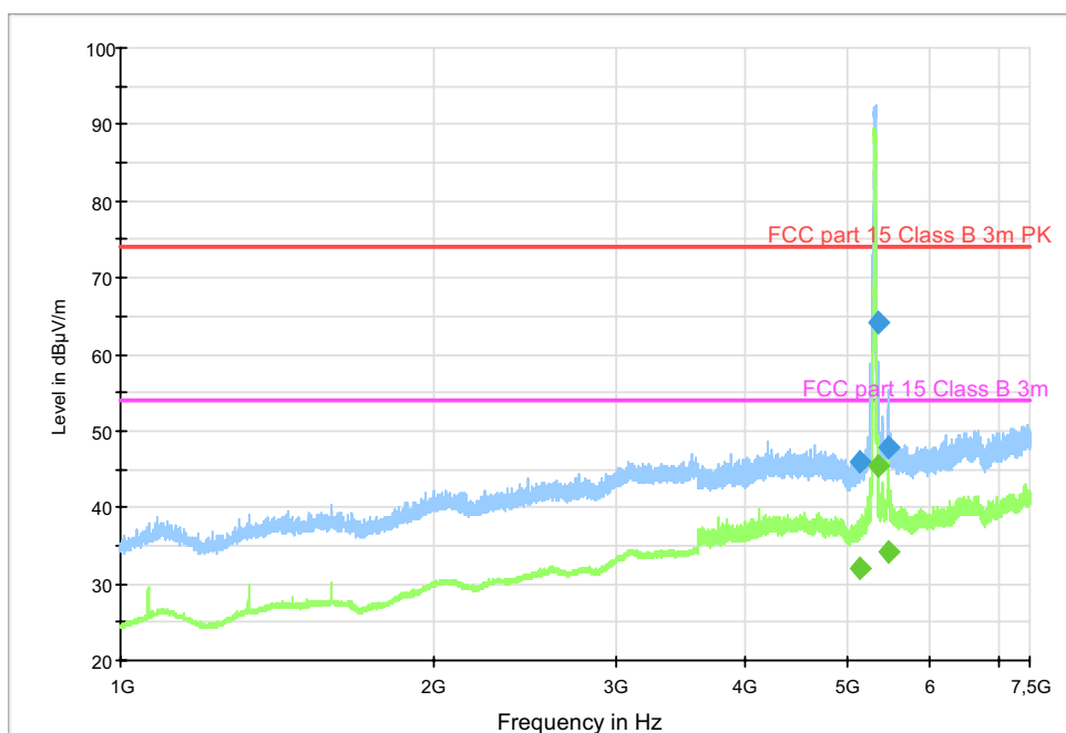
Diagram, Peak overview sweep, 1– 7,5 GHz at 3 m distance. TX channel 64 , EUT orientation 2.
