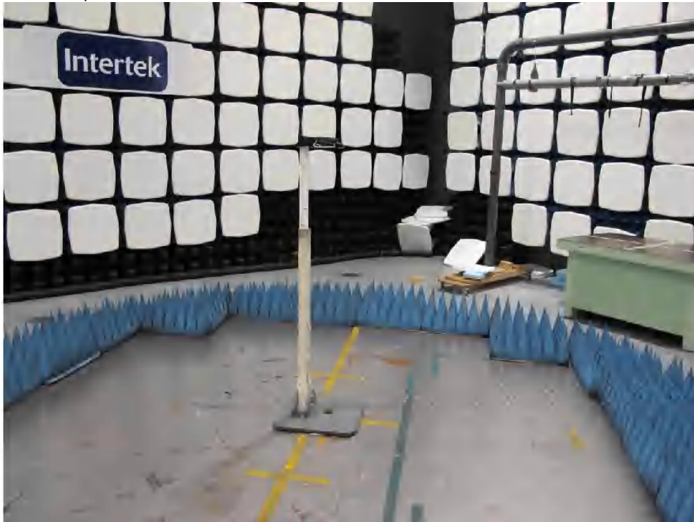
Test set up radiated emission > 1GHz
