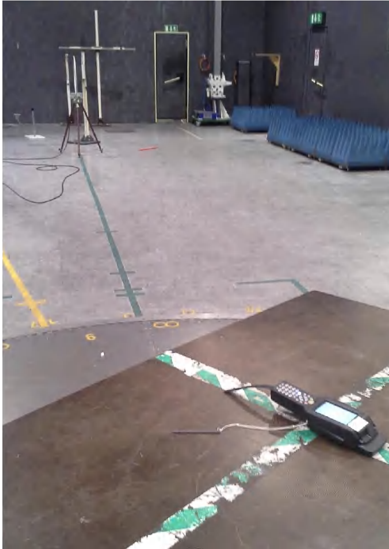
Test set up radiated emission 9 kHz – 30 MHz
