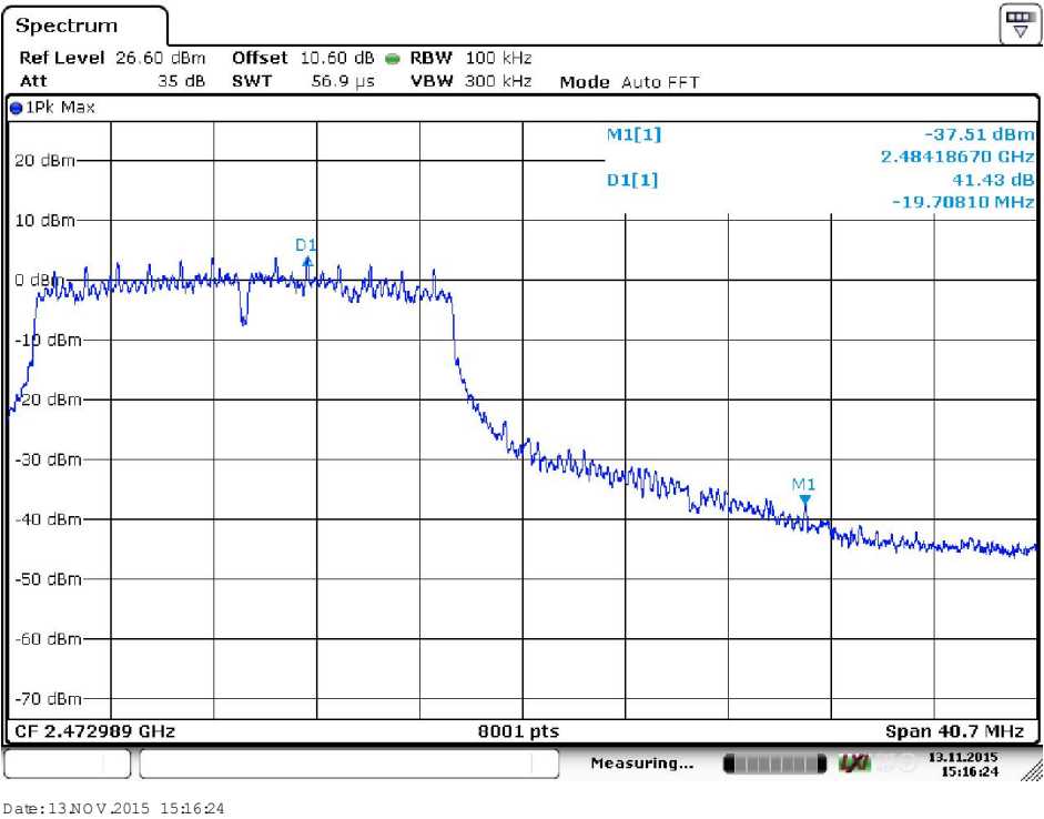
Screenshot: Upper band edge sweep, g
