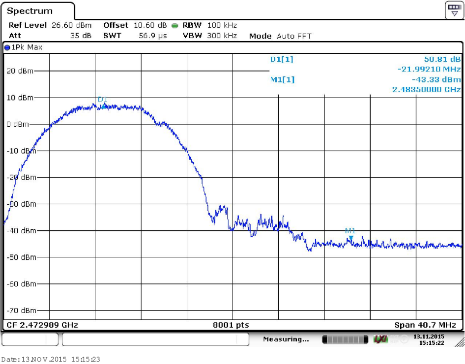
Screenshot: Upper band edge sweep, b mode
