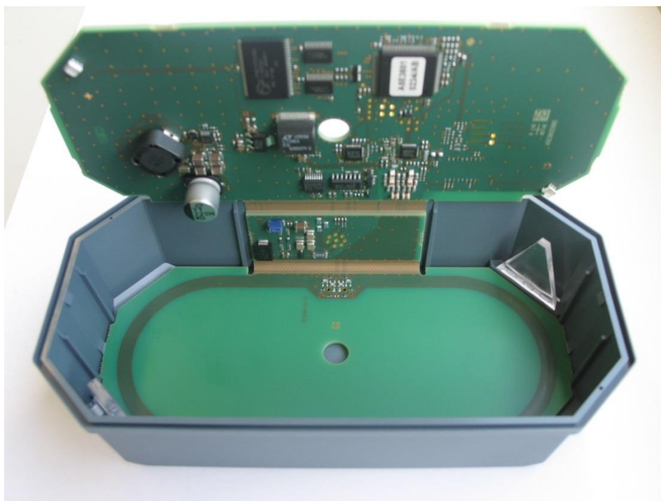
Fig. 3: PCB fixed in housing
