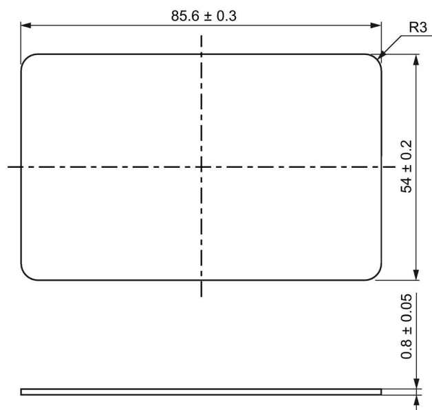
Figure 8-33 Dimensional drawing MDS D400 (dimensions in mm)
