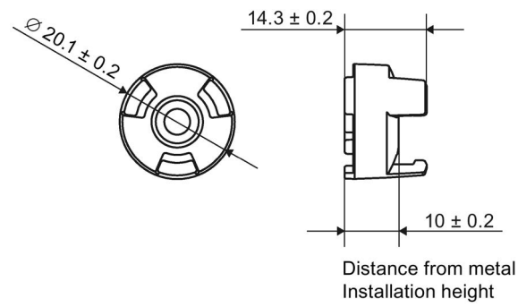
Figure A-8 Dimension drawing of spacer 6GT2690-0AG00
