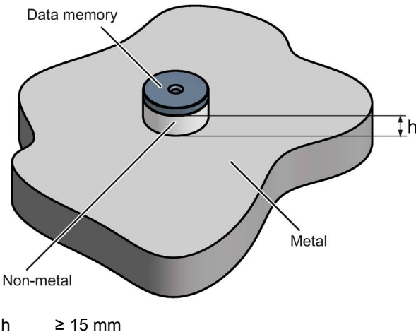
Figure 8-46 Mounting the MDS D124/D324/D424/D524/E624 and RF320T on metal with spacer
