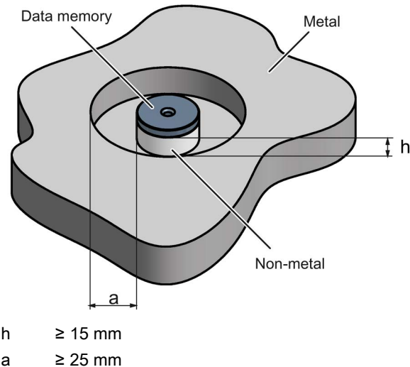
Figure 8-26 Flush-mounting of the MDS D124/D324/D424/D524/E624 and RF320T in metal with spacer
