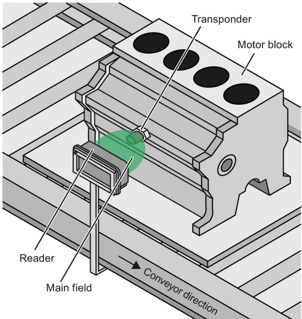
Figure 8-49 Application example
