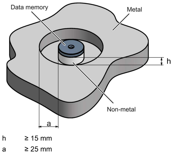
Figure 8-47 Flush-mounting of the MDS D124/D324/D424/D524/E624 and RF320T in metal with spacer
