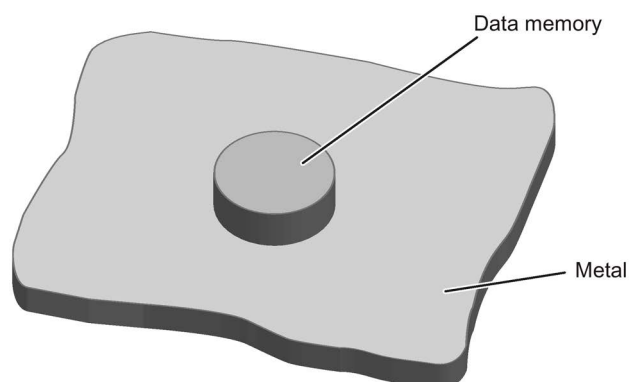
Figure 8-34 Mounting of MDS D421/D521/E623 on metal
