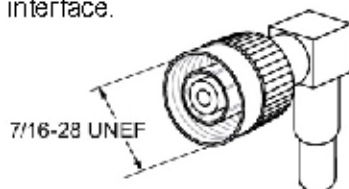
Figure 4-10 Thread standardization
