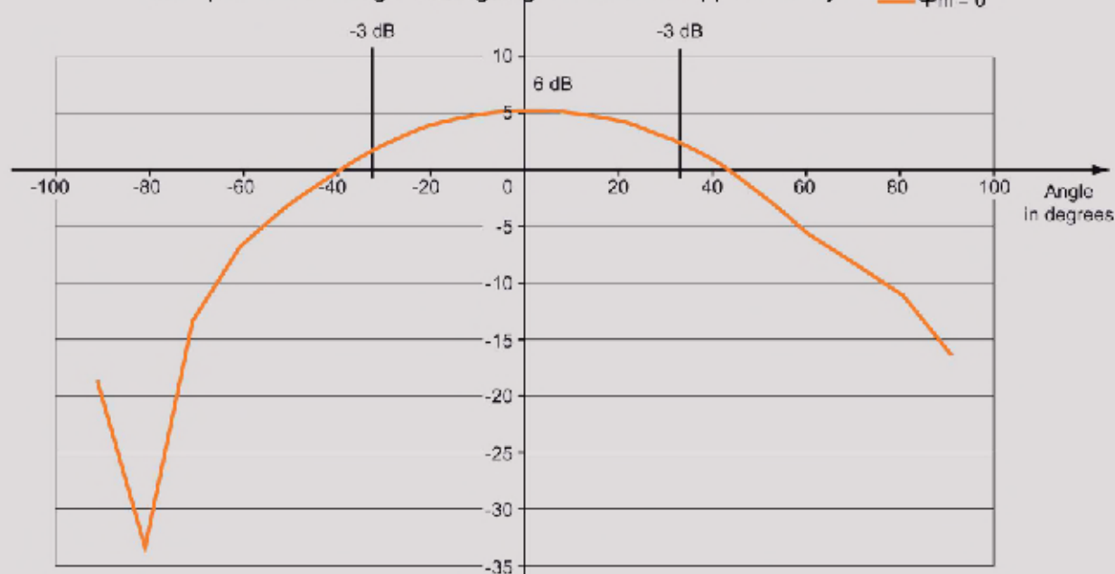
Figure 6-49 Directional radiation pattern of the antenna (at 865 MHz, horizontal alignment)
