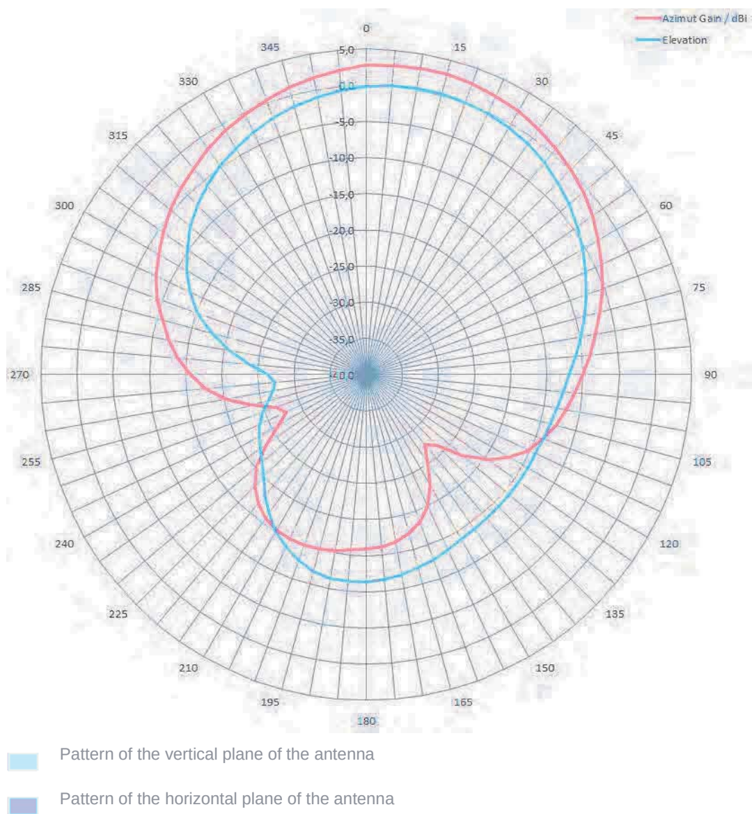
Figure 6-62 The RF680A directional radiation pattern in the FCC frequency band, axis of symmetry of the antenna, and polarization axis of the transponder are aligned vertically
