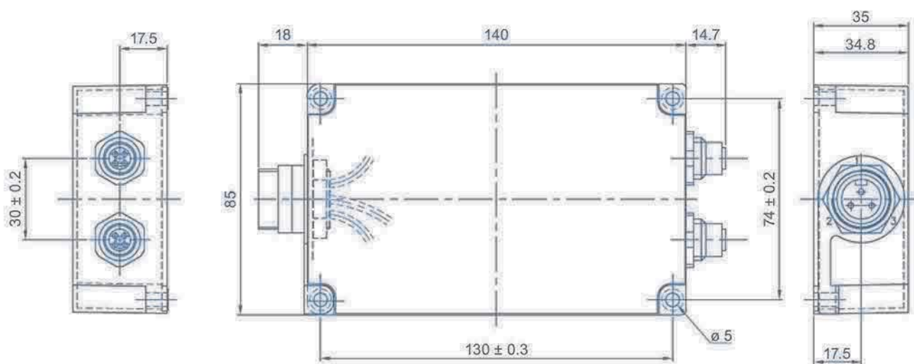
Figure 10-1 Dimension drawing wide-range power supply unit for SIMATIC RF systems
