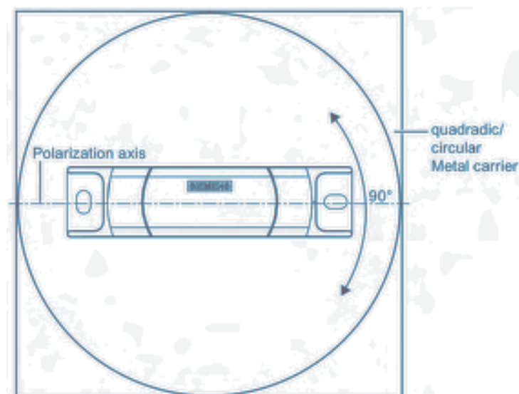
Figure 7-40 Optimum positioning of the transponder on a (square or circular) metal plate
