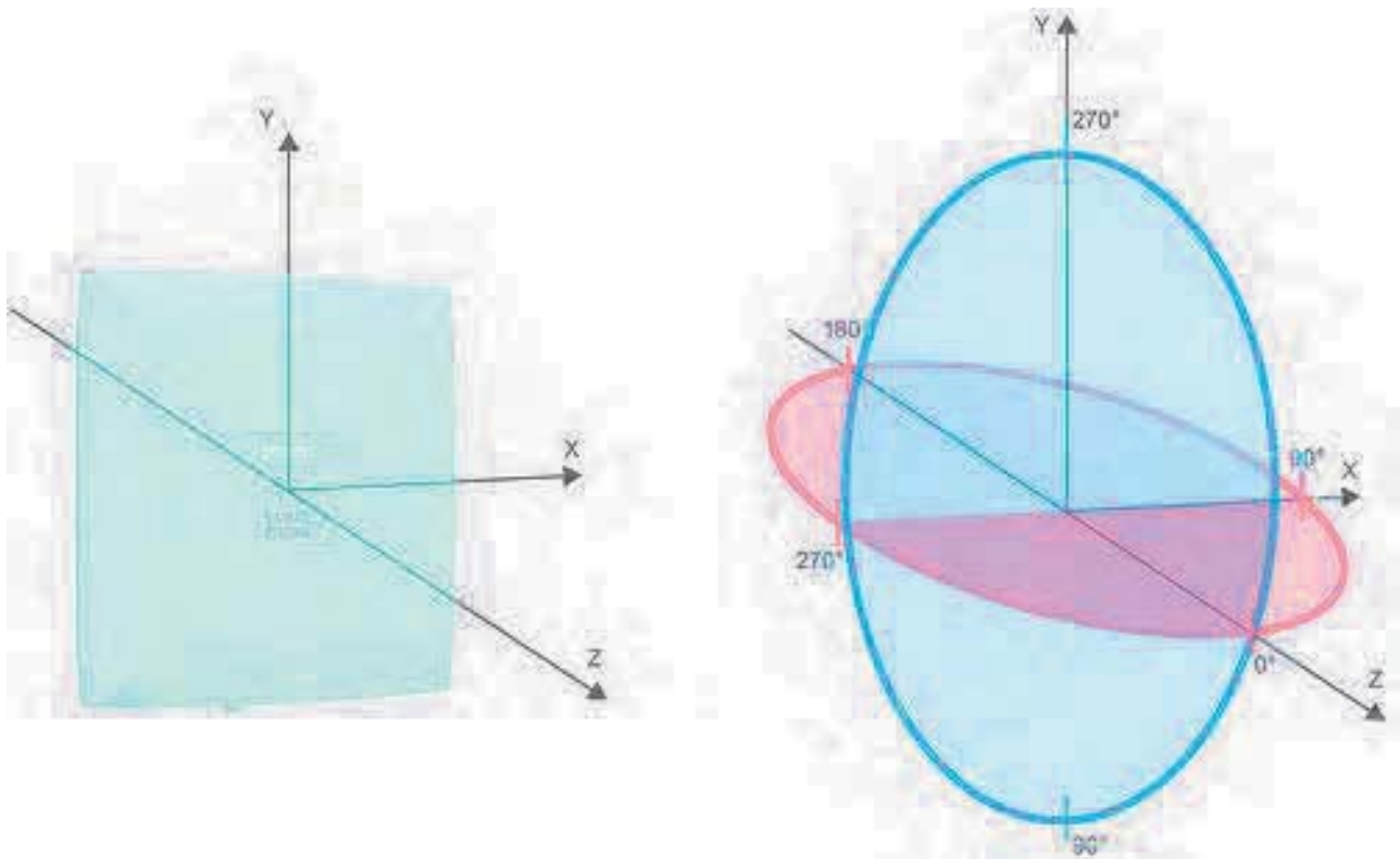
Figure 6-42 Reference system
