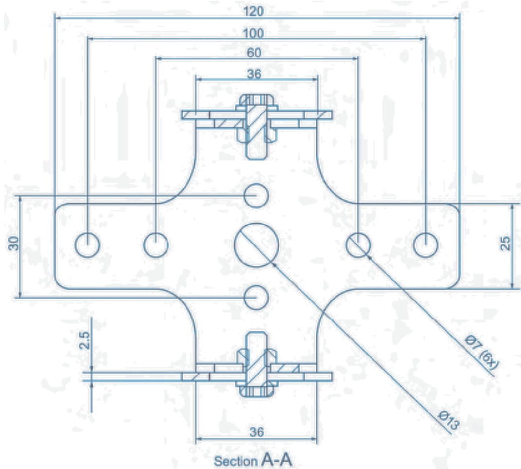
Figure 10-7 Section A-A
