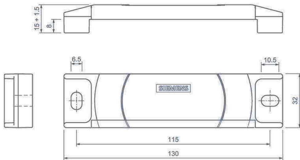
Figure 7-41 Dimension drawing of SIMATIC RF682T
