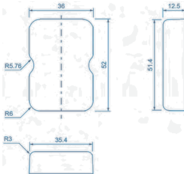
Figure 7-31 Dimension drawing of SIMATIC RF645T
