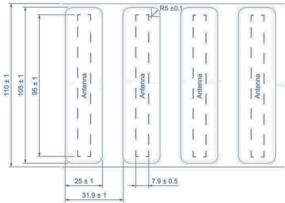
Figure 7-9 Dimension drawing SIMATIC RF630L (6GT2810-2AE80-0AX2)
