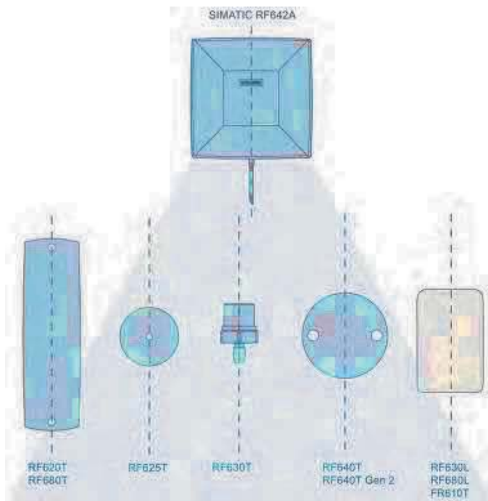
Figure 6-33 Antenna/transponder alignment
