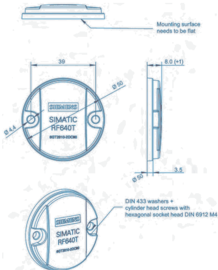
Figure 7-30 SIMATIC RF640T
