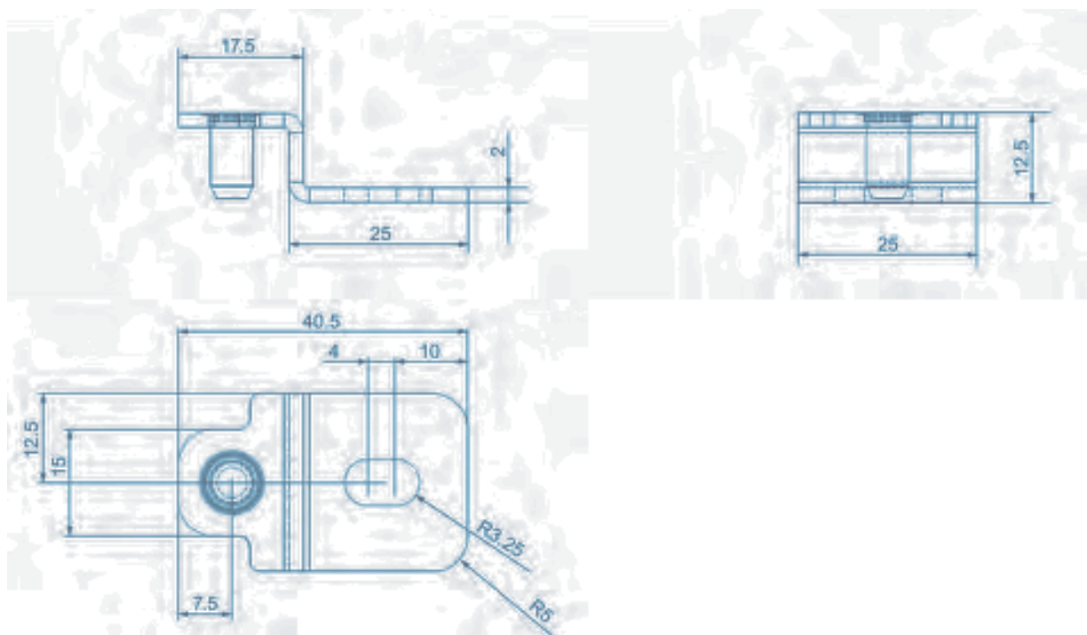
Figure 7-42 Dimension drawing mounting for SIMATIC RF68xT
