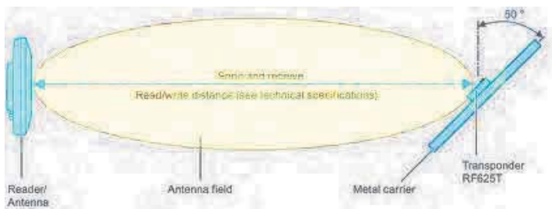
Figure 7-19 Example of optimum reader/antenna transponder positioning
