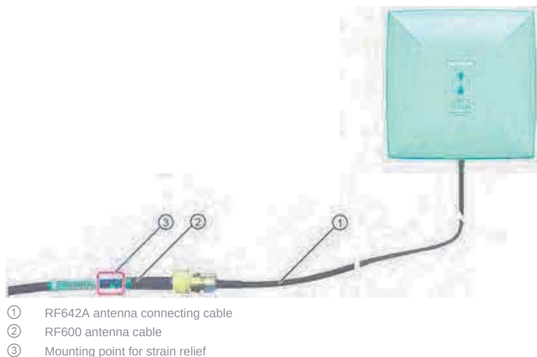
Figure 6-31 Strain relief
