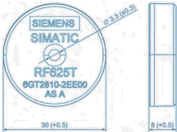
Figure 7-22 SIMATIC RF625T UHF Disk Tag
