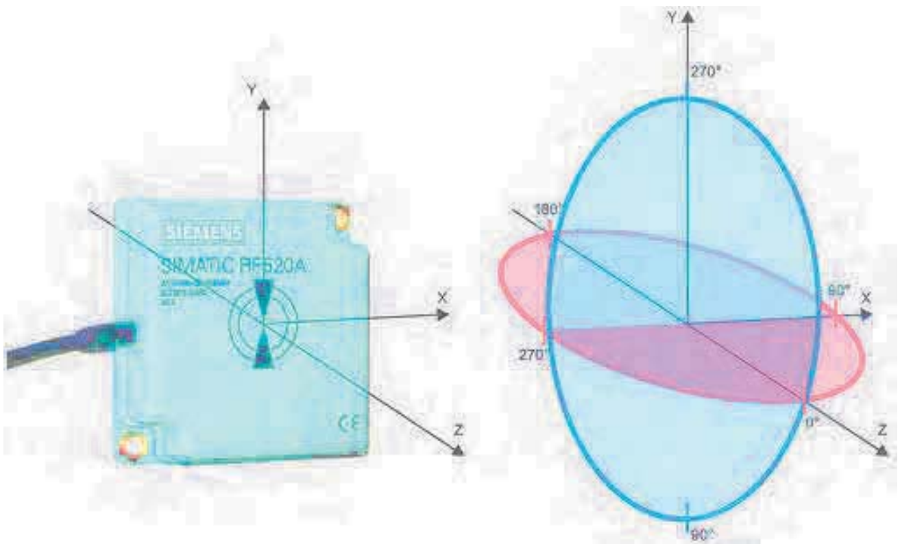
Figure 6-19 Reference system
