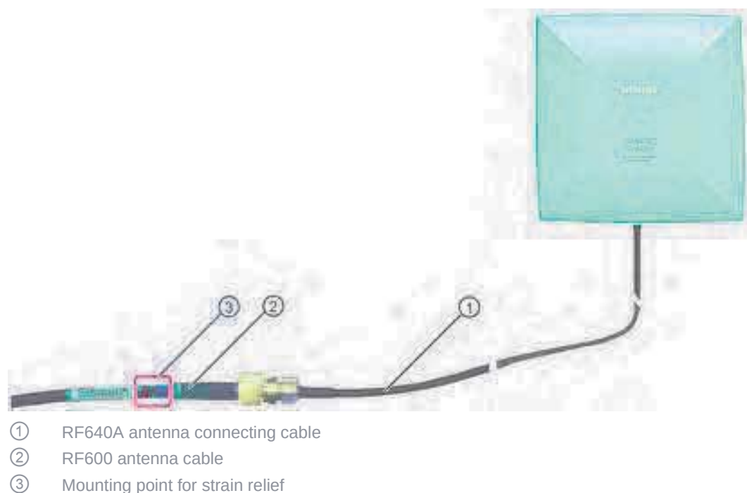
Figure 6-23 Strain relief
