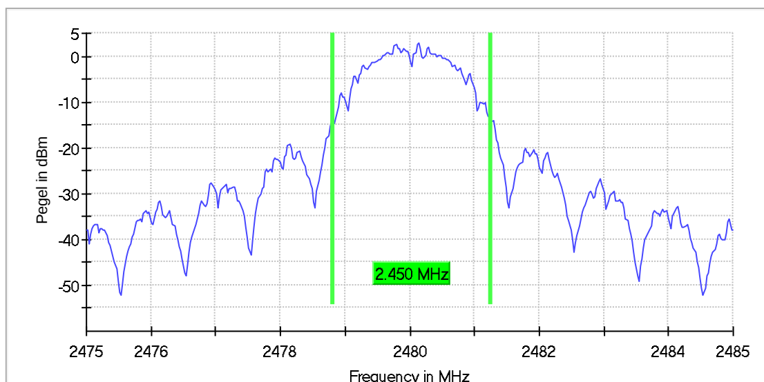
Figure 11 - 2480 MHz – 99% Bandwidth
