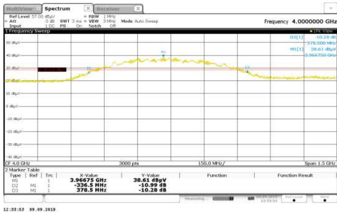
Figure 4 – -10 dB bandwidth, Channel 2
