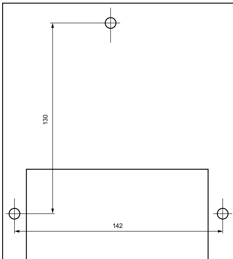
Figure 6-6 Drilling pattern - All dimensions specified in millimeters.
