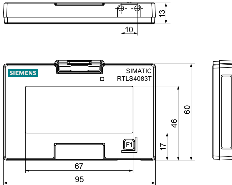
Figure 7-3 Dimension drawing SIMATIC RTLS4083T - All dimensions specified in millimeters
