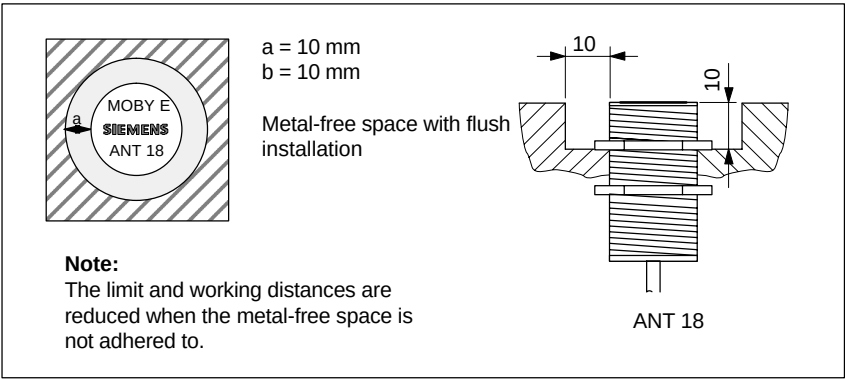
Figure 5-27 Metal-free space for the ANT 18
