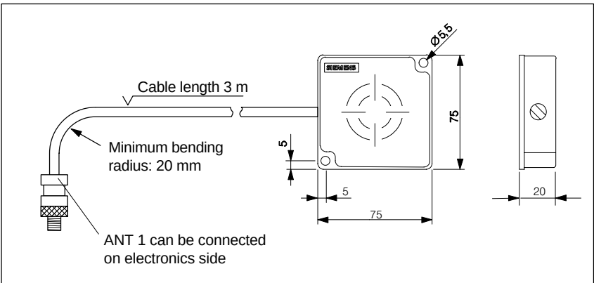
Figure 5-34 Dimensioned drawing of the ANT 1
