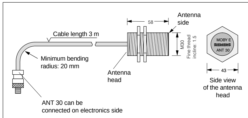
Figure 5-37 Dimensioned drawing of the ANT 30
