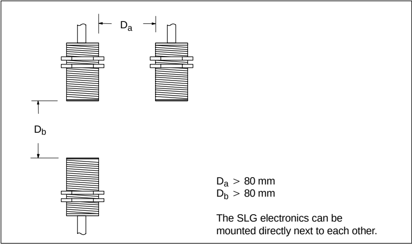
Figure 5-30 Distance D: ANT 12
