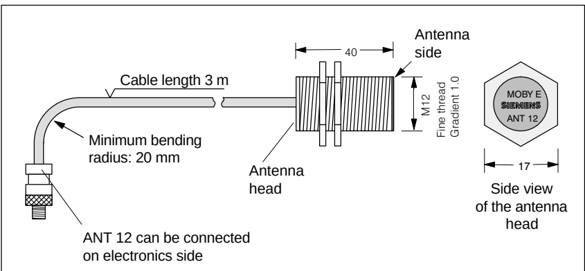
Figure 5-35 Dimensioned drawing of the ANT 12
