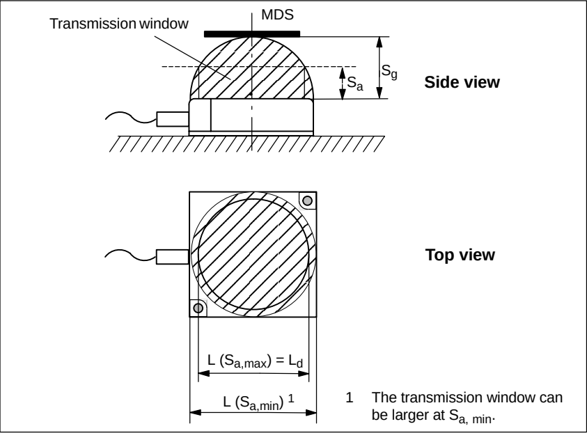
Figure 5-21 Transmission window of the ANT 1
