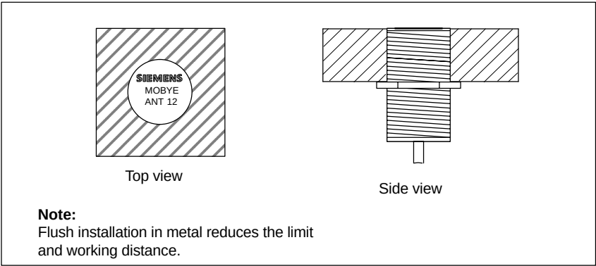
Figure 5-26 Metal-free space for the ANT12
