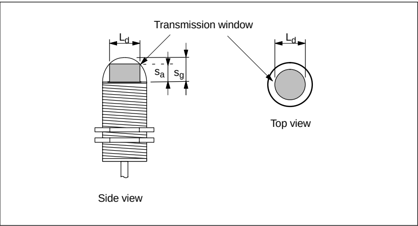
Figure 5-22 Transmission window of the ANT12
