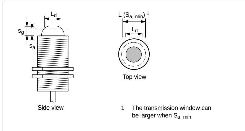
Figure 5-23 Transmission window of the ANT18
