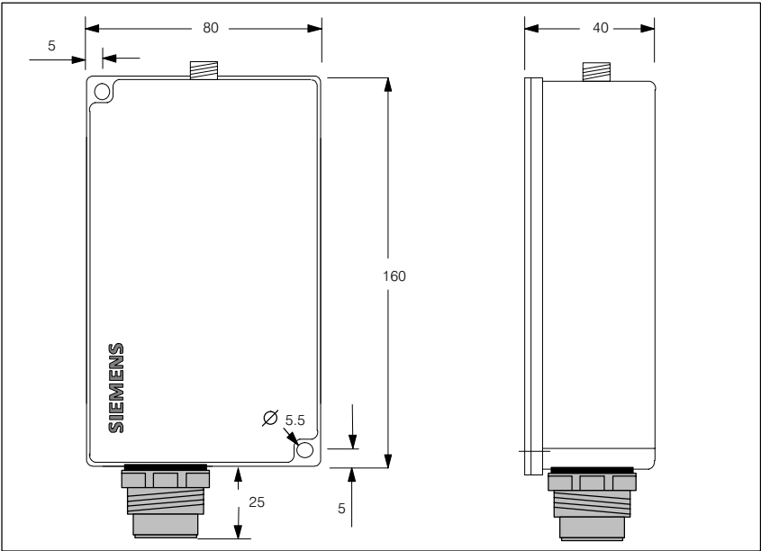
Figure 5-33 Dimensioned drawing of SLG 75
