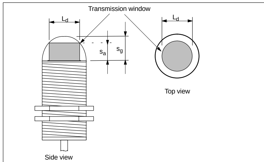
Figure 5-24 Transmission window of the ANT 30
