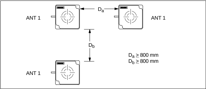
Figure 5-29 Distance D: ANT 1
