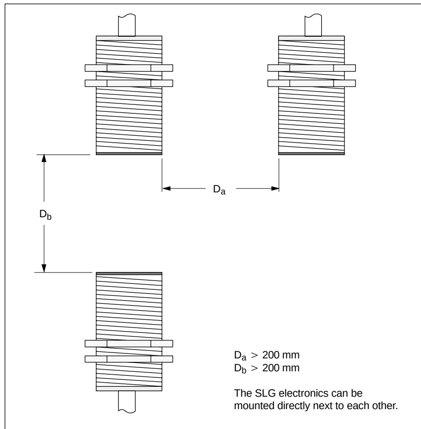
Figure 5-32 Distance D: ANT 30
