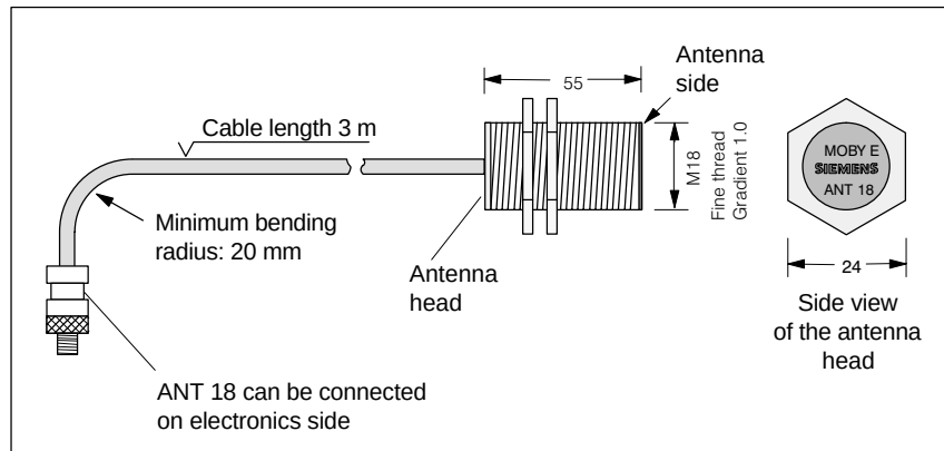
Figure 5-36 Dimensioned drawing of the ANT 18
