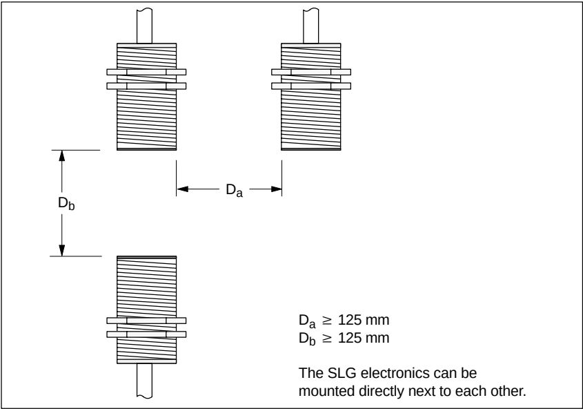
Figure 5-31 Distance D: ANT 18
