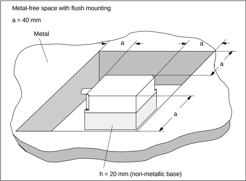
Figure 5-25 Metal-free space for the ANT 1
