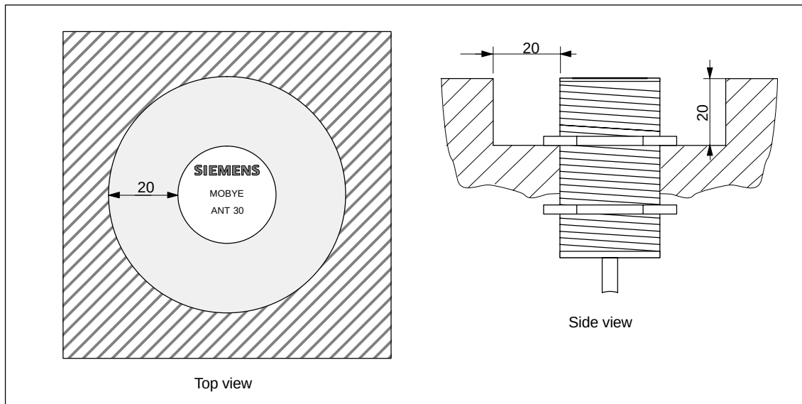
Figure 5-28 Metal-free space for the ANT 30
