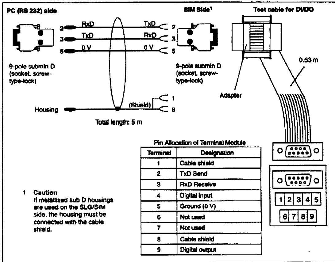
Figure 3-31 Connection cable: PC ↔ SIM
