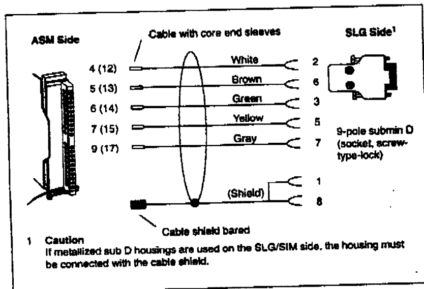
Figure 3-30 Connection cable: ASM 470 ↔ SLG
