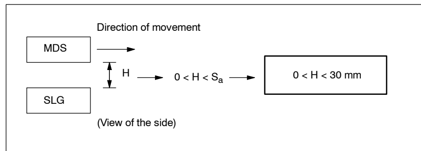
Figure 3-6 Tolerances of the height allowance of the pallet
