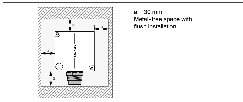
Figure 5-19 Metal-free space for SLG 42
