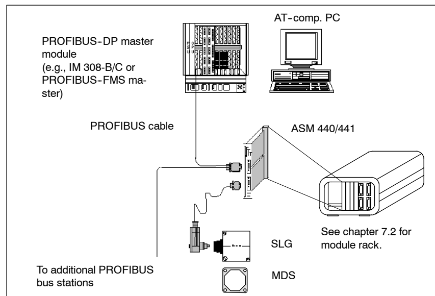
Figure 6-25 Configurator for ASM 440/441
