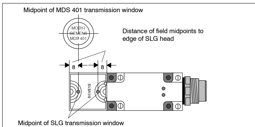
Figure 4-9 Definition of the field midpoints of SLG 41
