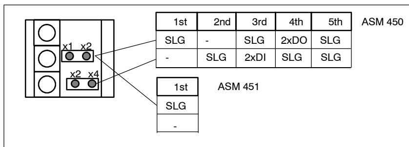
Figure 6-32 SLG and DI/DO configuration for ASM 450/451
