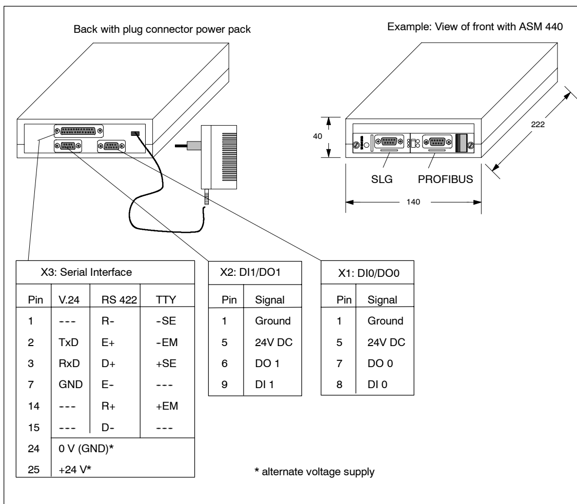
Figure 7-3 Plug connector assignment and dimensions
