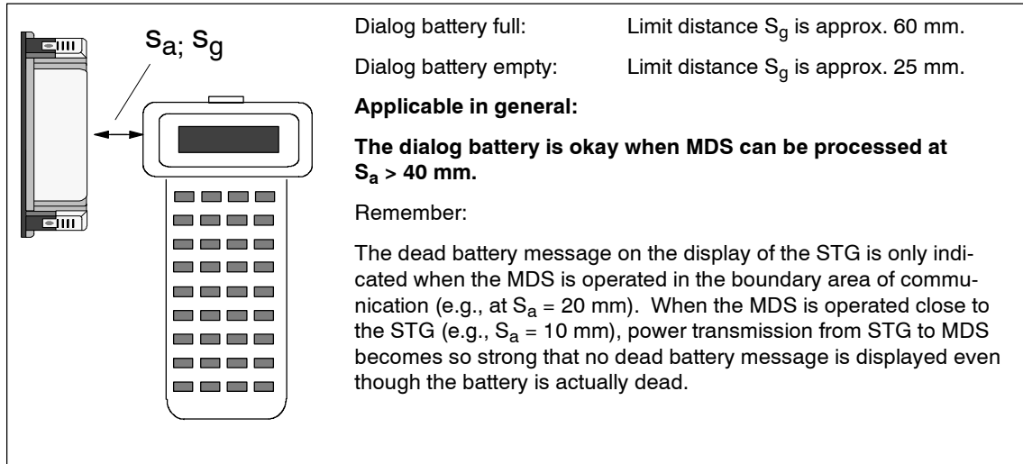
Figure 3-30 Dead battery measurement with the STG
