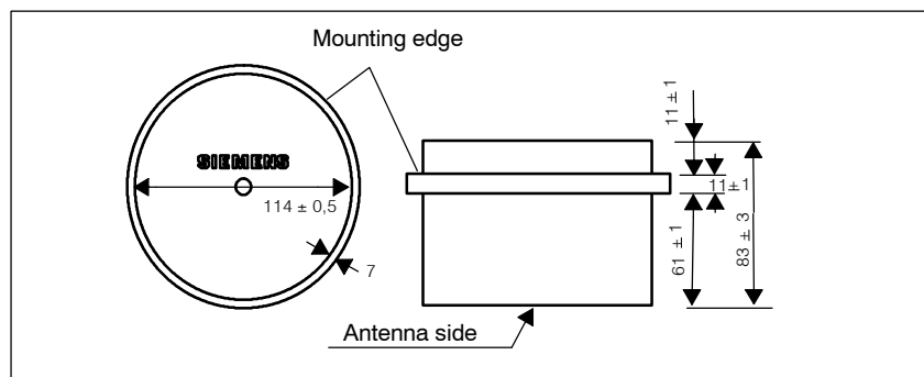
Figure 4-34 Dimensional drawing of MDS 439 E
