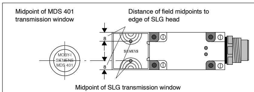
Figure 4-11 Definition of the field midpoints of SLG 41-S
