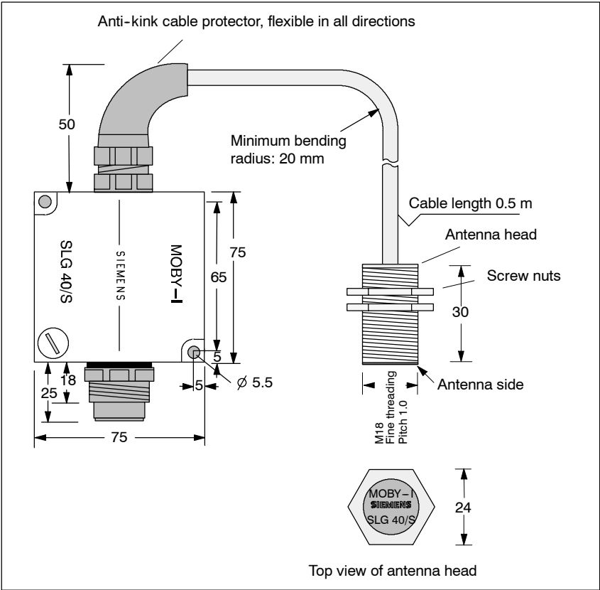
Figure 5-10 Dimensional diagram of SLG 40-S
