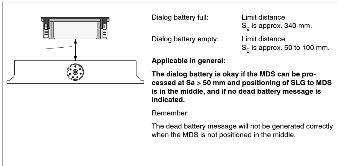
Figure 3-31 Dead battery message with SLG 43
