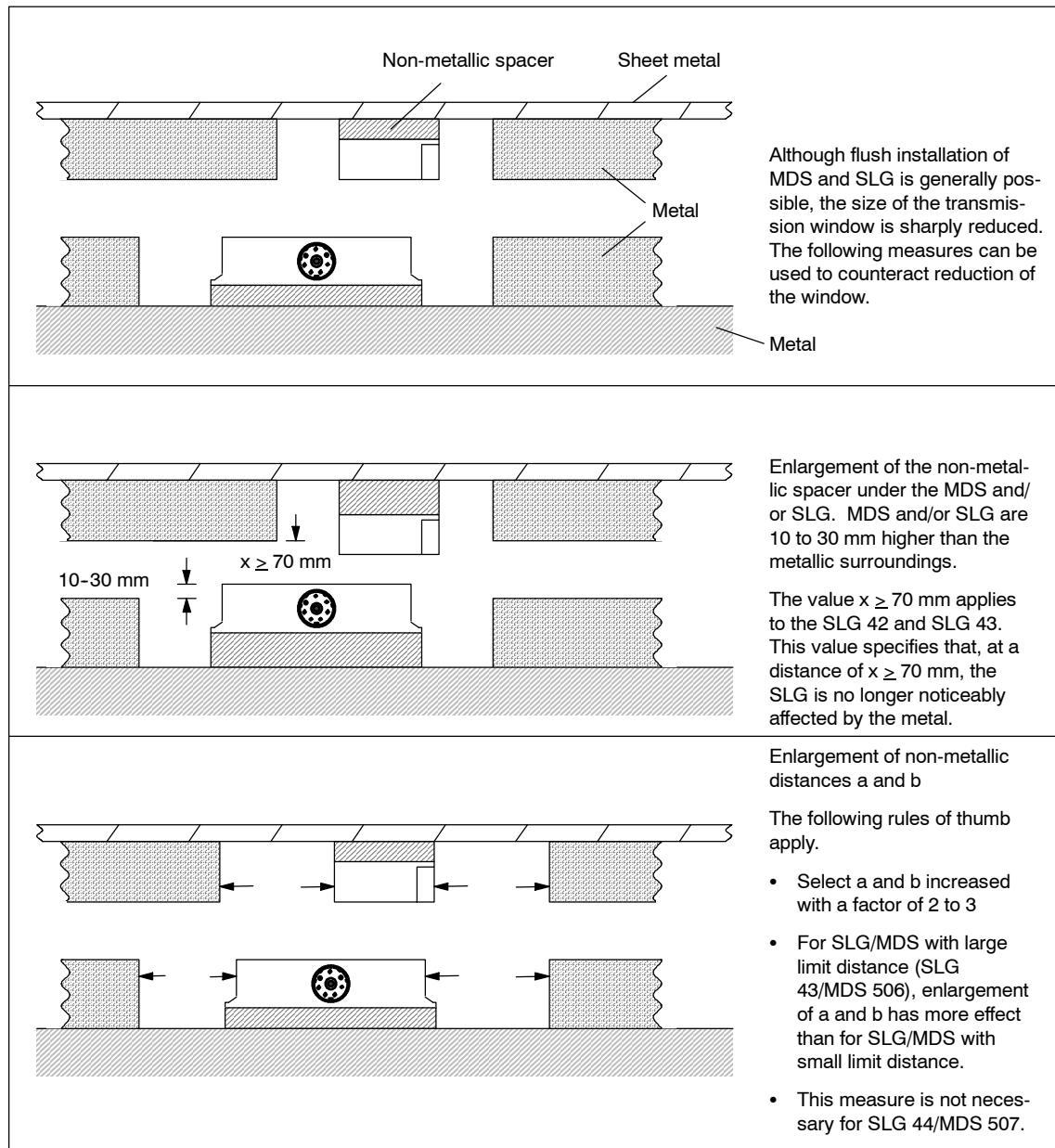
Figure 3-20 Flush installation
