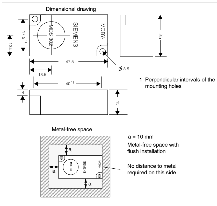
Figure 4-4 Dimensions of MDS 302
