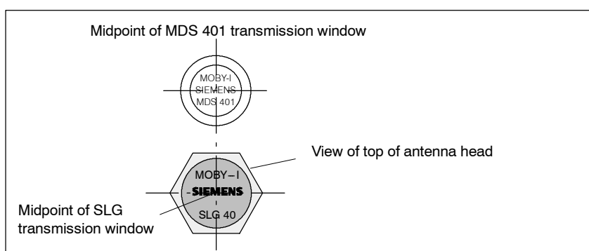
Figure 4-10 Definition of the field midpoints of SLG 40
