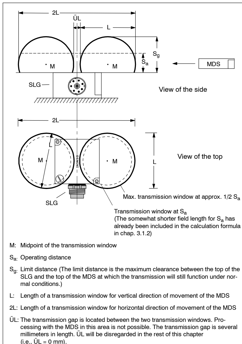
Figure 3-1 Transmission window
