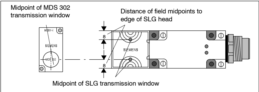
Figure 4-7 Definition of the field midpoints of SLG 41-S
