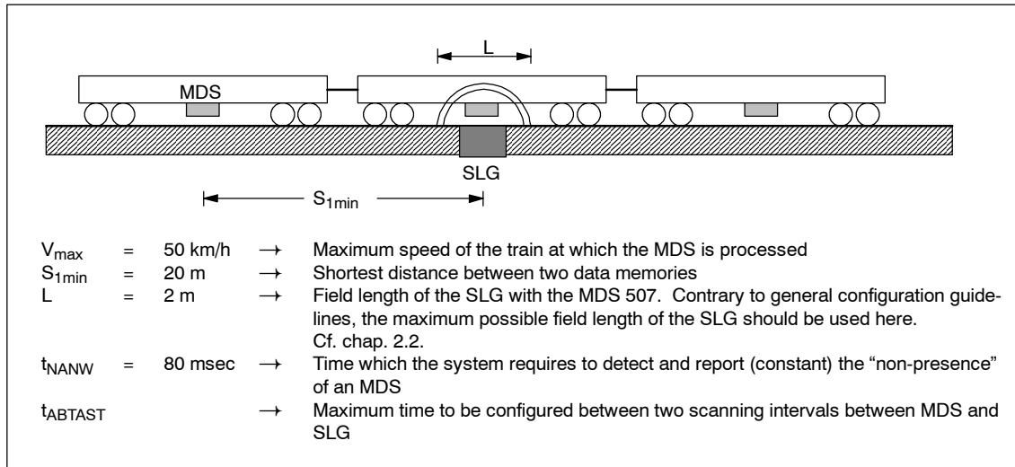
Figure 3-21 Sample configuration of t_{ABTAST} : Train with several cars
