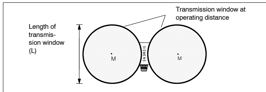
Figure 5-23 Transmission window of SLG 43
