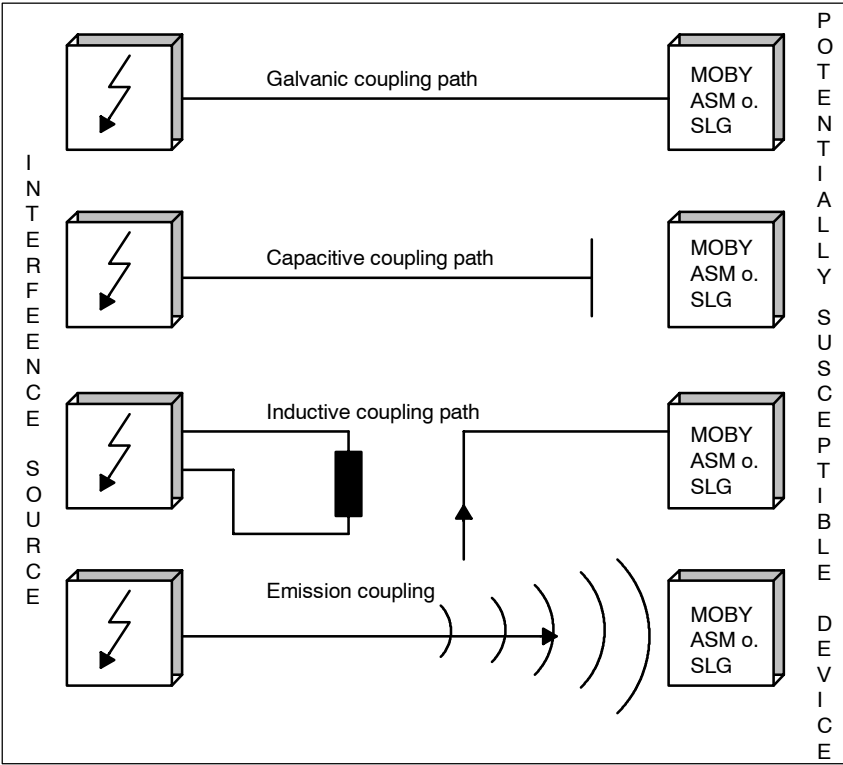
Figure 3-41 The four kinds of interference coupling
