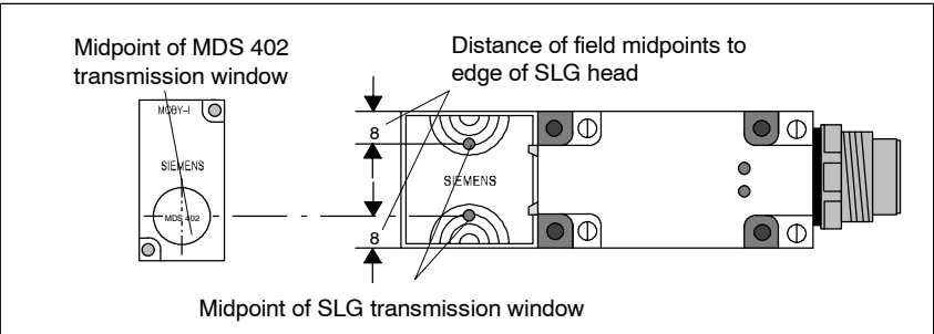
Figure 4-16 Definition of the field midpoints of SLG 41-S
