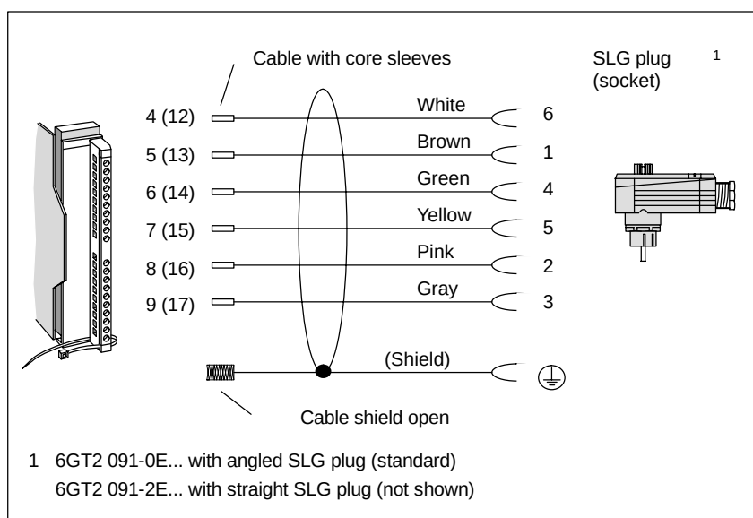
Figure 3-16 Connection cable ASM 475 ↔ SLG U92 with RS 422
