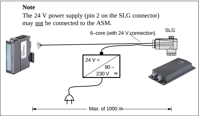
Figure 3-13 SLG with extra power pack
