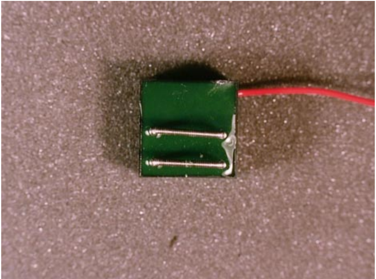
External photo TranX 120 (bottom)
