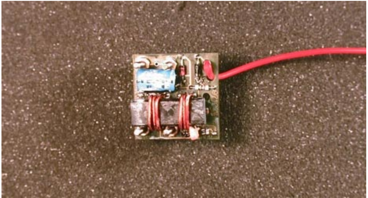
Internal photo TranX 120 (top)
