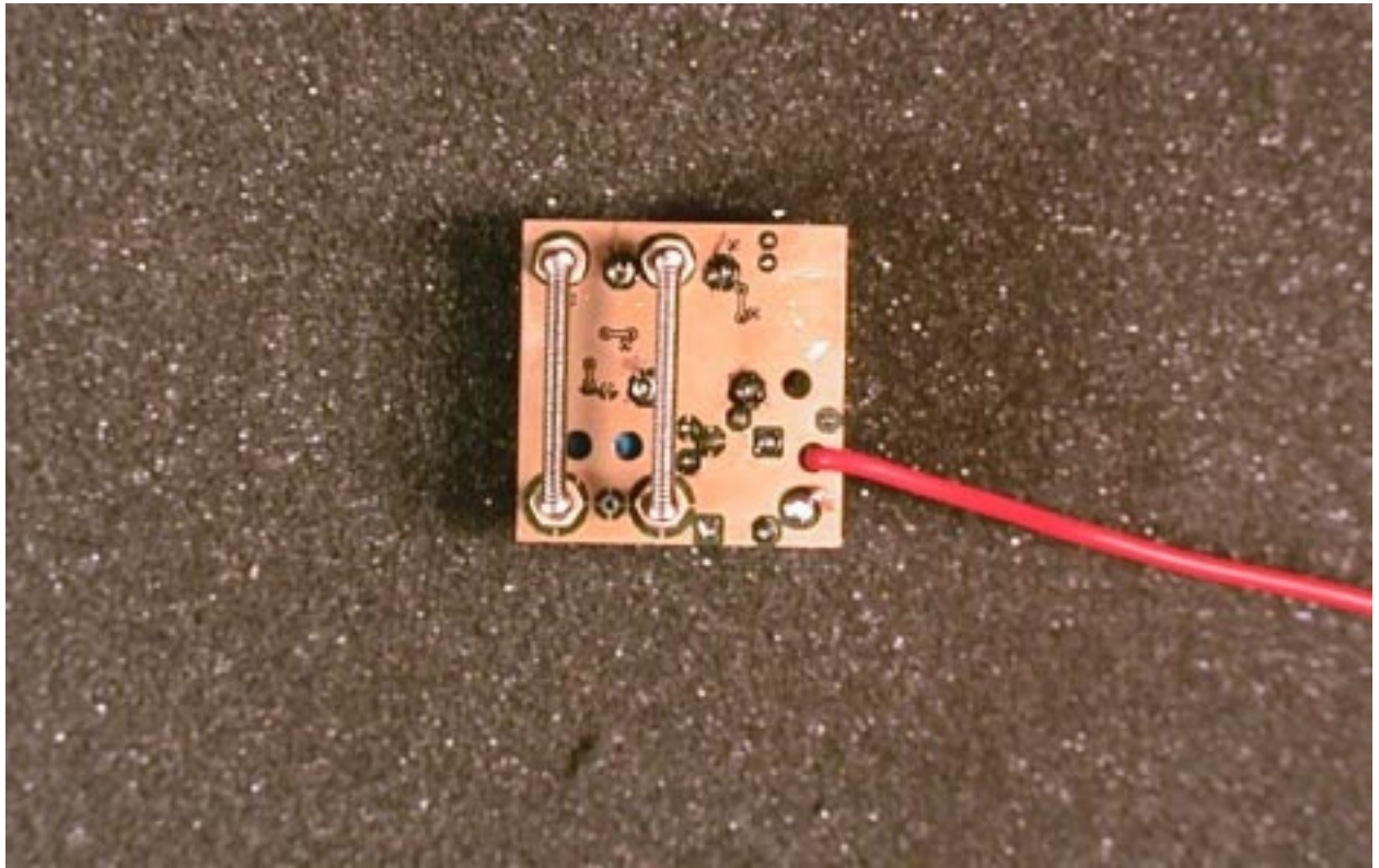
Internal photo TranX 120 (bottom)
