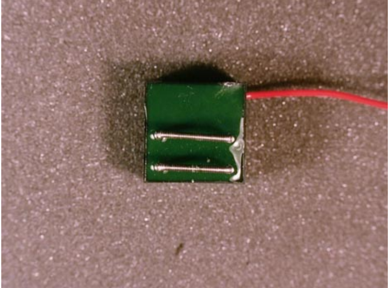
External photo TranX 120 (bottom)
