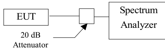
Figure 4: Emission bandwidth measurement configuration.
