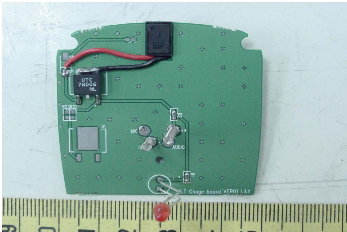
Component View of Main PCB (Charger)
