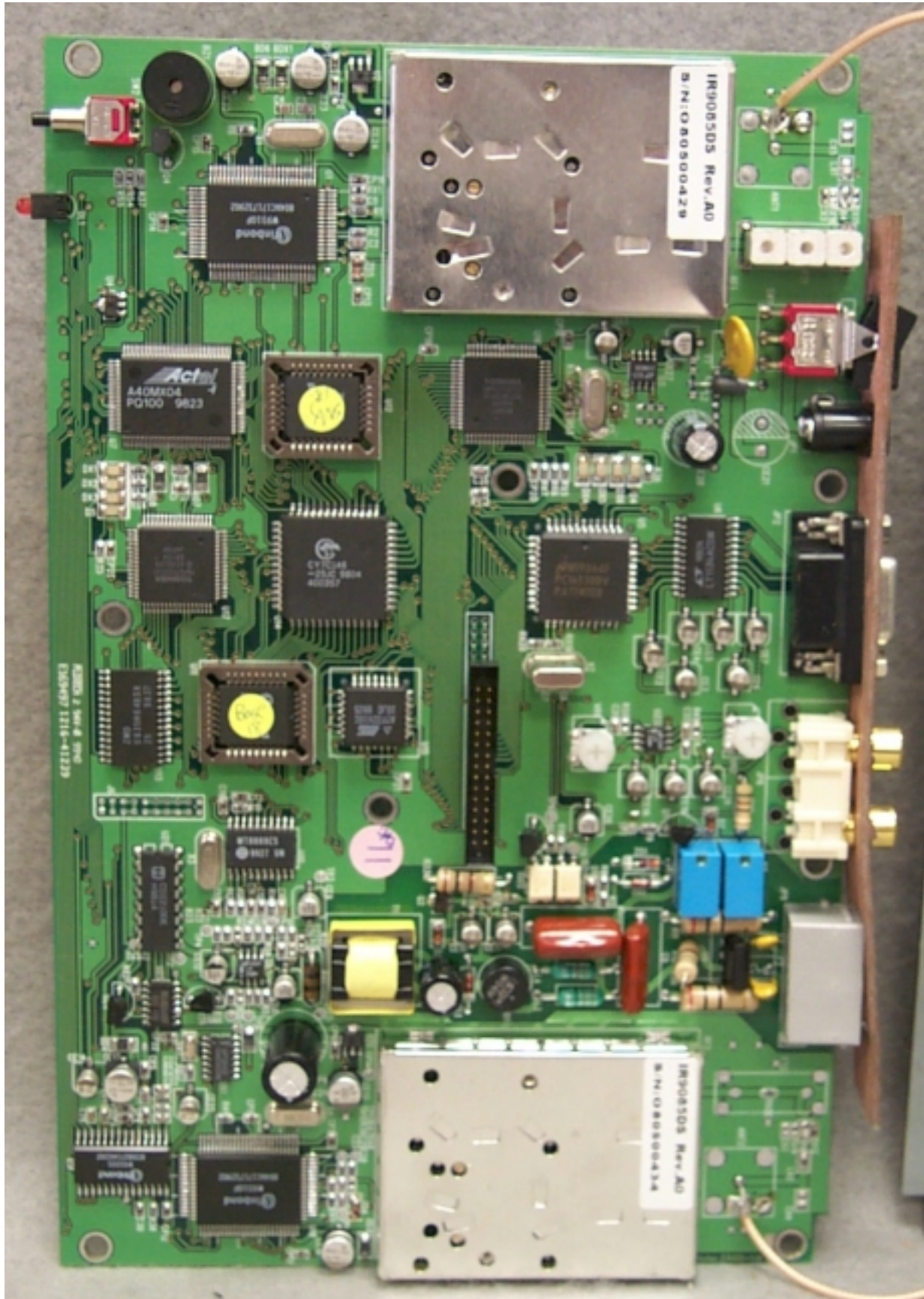
Photo 3. EUT, Top View of Main Board
