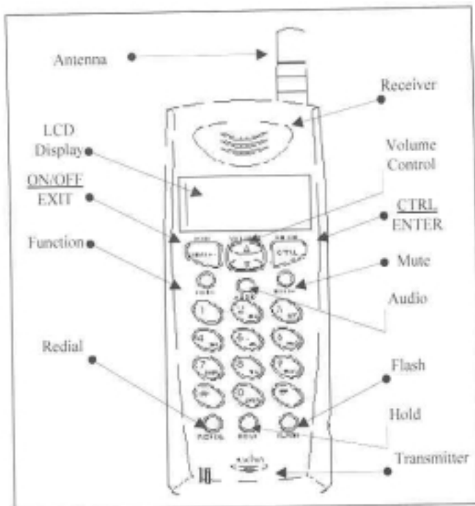
Figure 2.3 Mobile Unit
