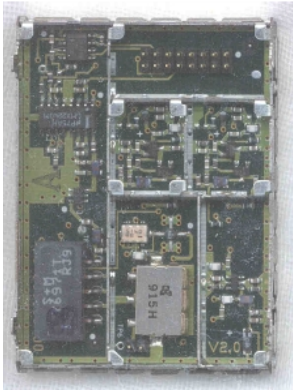
Photo 9. EUT, Bottom View of Transceiver Board (Shield Removed)
