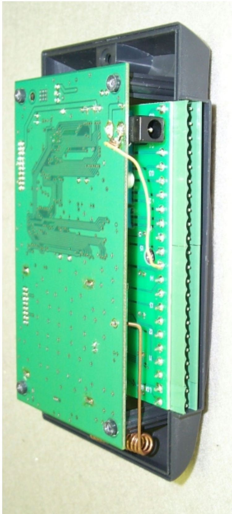
Photo 10. EUT, View Showing Added Wire Jumper
