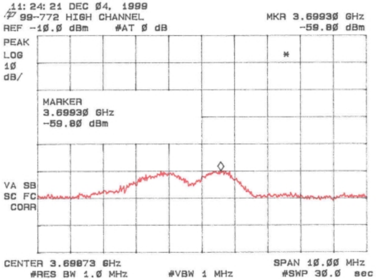
Figure 5l Peak Radiated Spurious Emission 15.247(c) High
