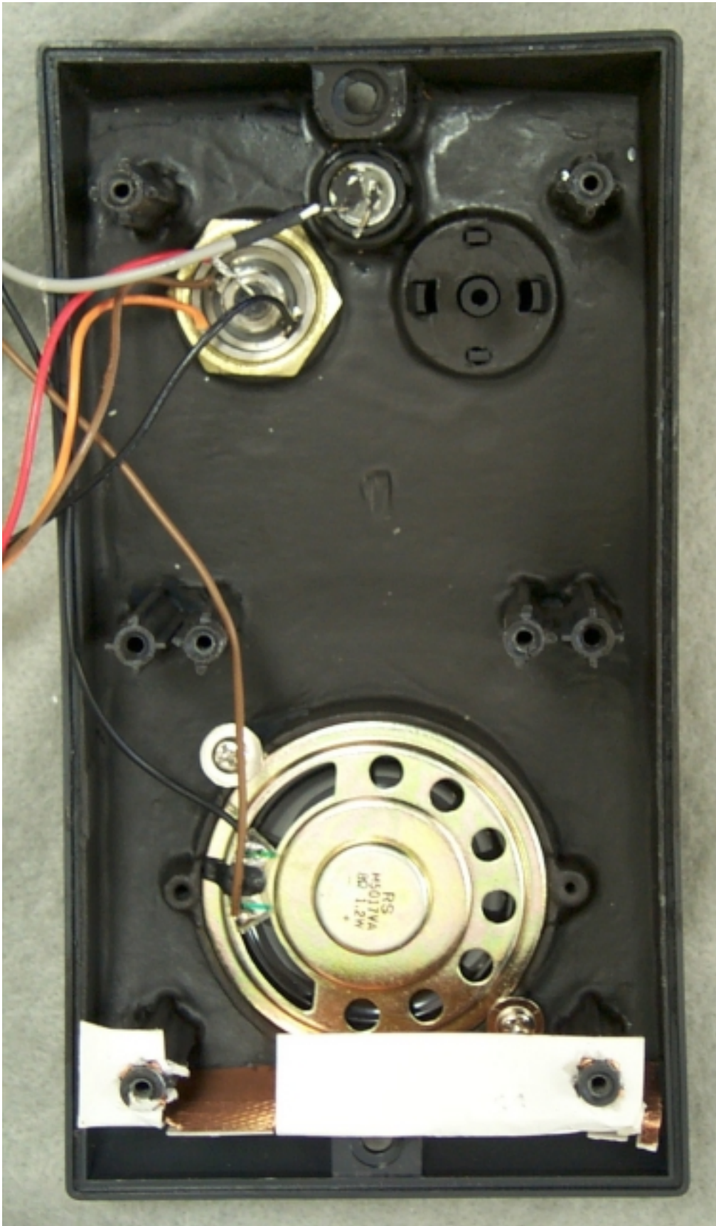
Photo 6. EUT, View of Bottom Side of Case with Board Removed
