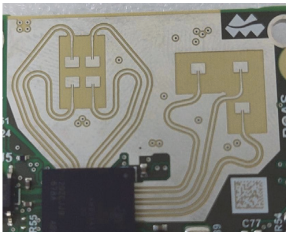
Antenna Photo
