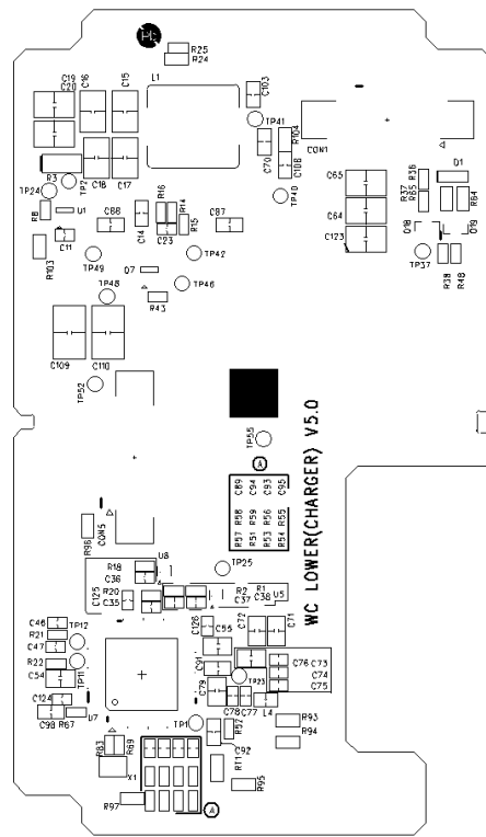
SILKSCREEN TOP
