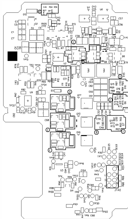
SILKSCREEN BOTTOM
