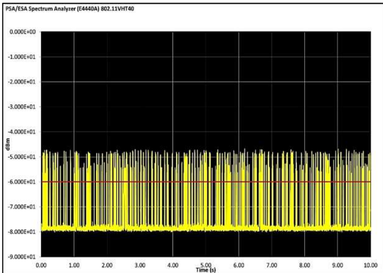
7.7 Channel Loading_801.11VHT40_8192pt_7Mbps
