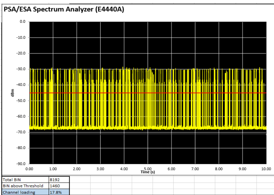
7.7 Channel Loading_801.11HT80_8192pt_8Mbps
