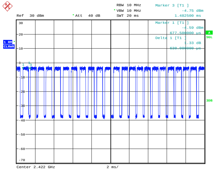
Test Graph_IEEE802.11 n (HT40) SISO Duty Cycle:
