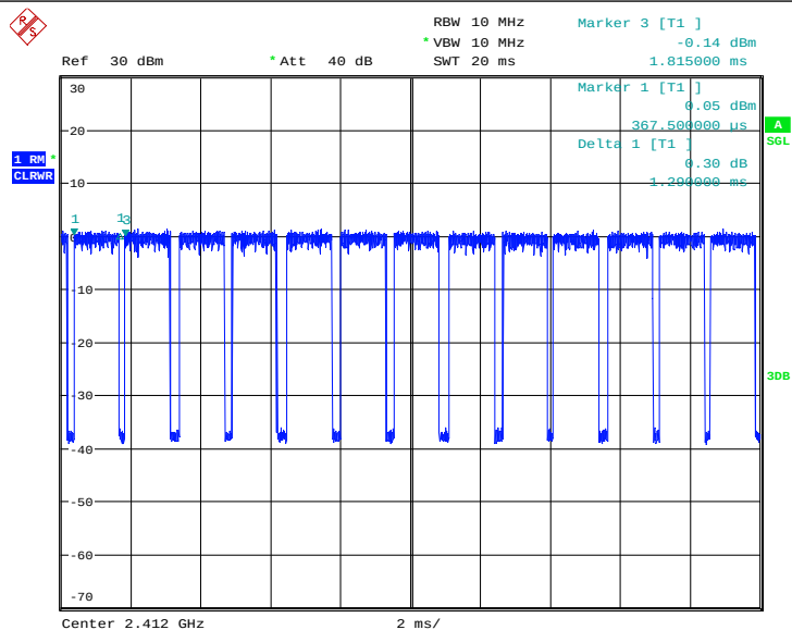
Test Graph_IEEE802.11 n (HT20) SISO Duty Cycle:
