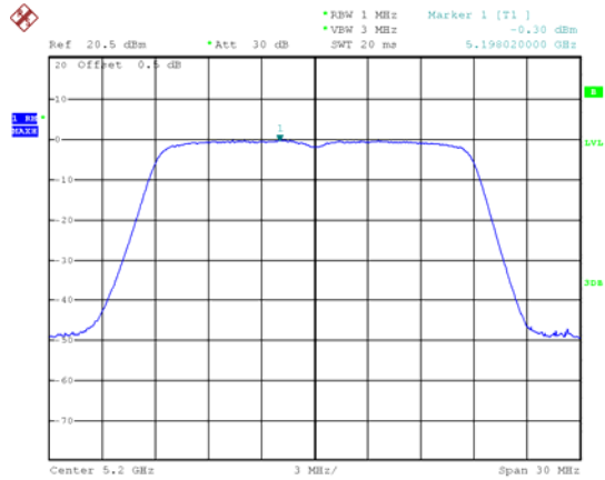
802.11ac VHT20 Middle channel
