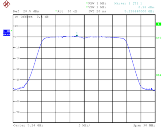
802.11ac VHT20 High channel
