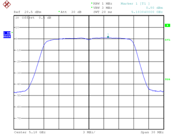
802.11ac VHT20 Low channel
