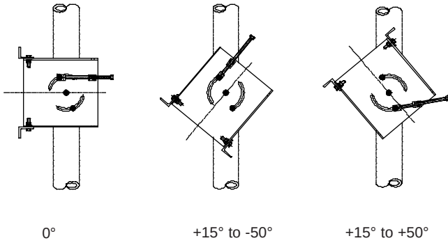
Elevation Adjustment Ranges
