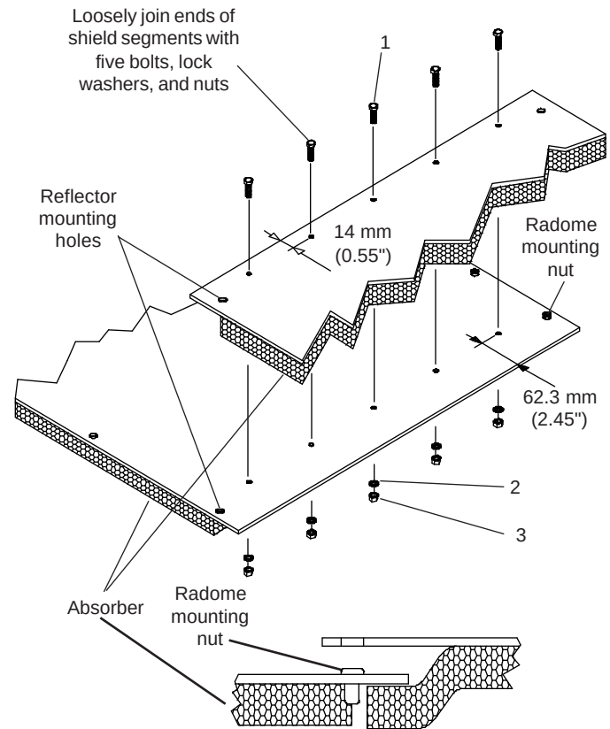
Typical overlap arrangement
