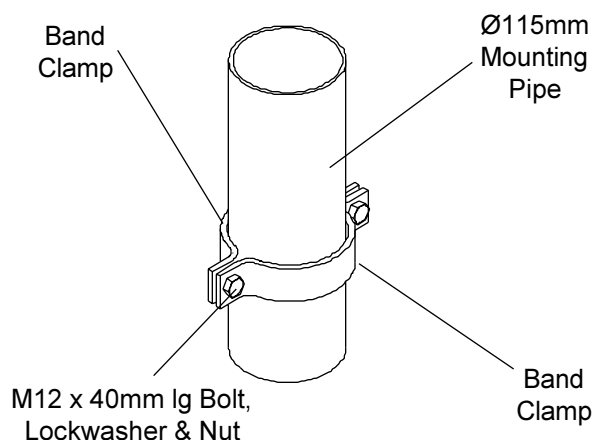
Figure 6. Attachment of Antenna Support Clamp
