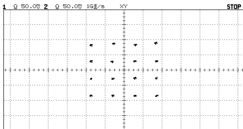
Figure 2-2 16 QAM Constellation
