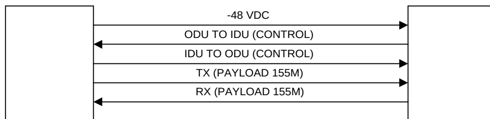
Figure 2-3 Signal Direction Through the Coaxial Cable
