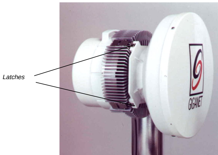
Figure 2-4 ODU Mounted on the Antenna
