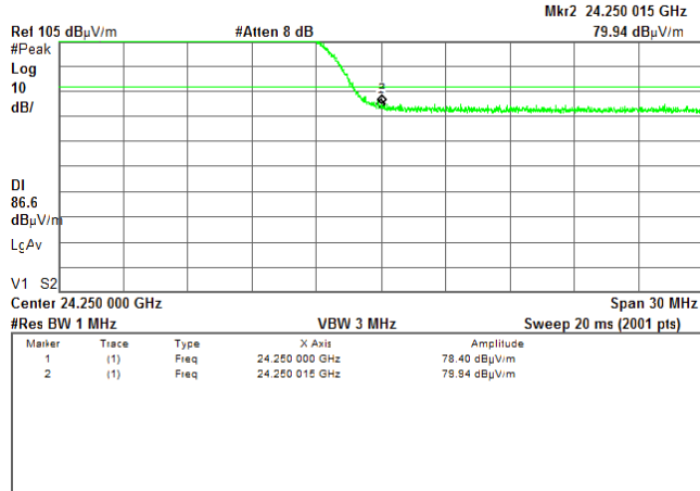
Plot 7.5.24 High band edge emission test result
