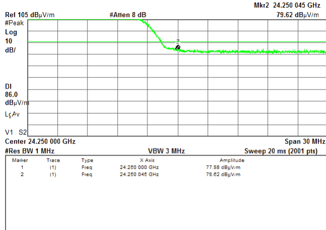
Plot 7.5.30 High band edge emission test result
