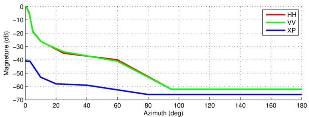
0.3m 17.70-19.70 GHz RADIATION PATTERN ENVELOPE
