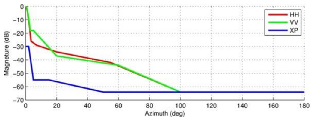
0.3m 27.50-29.60 GHz RADIATION PATTERN ENVELOPE
