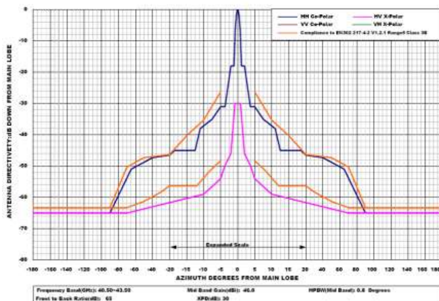
0.6m 40.50-43.50GHz HH&HV RADIATION PATTERN ENVELOPE
