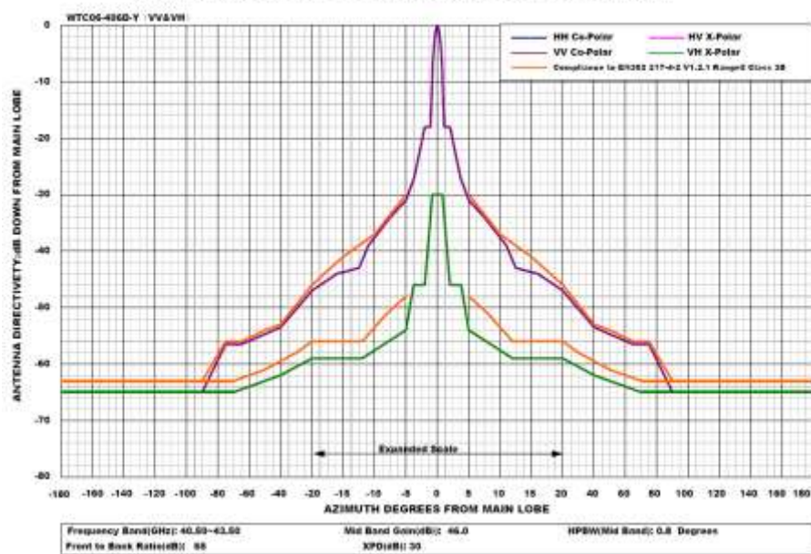
0.6m 40.50-43.50GHz VV&VH RADIATION PATTERN ENVELOPE
