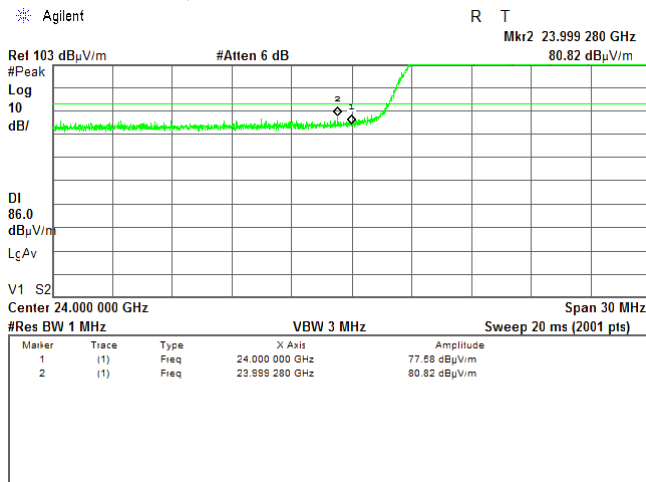
Plot 7.4.14 Low band edge emission test result
