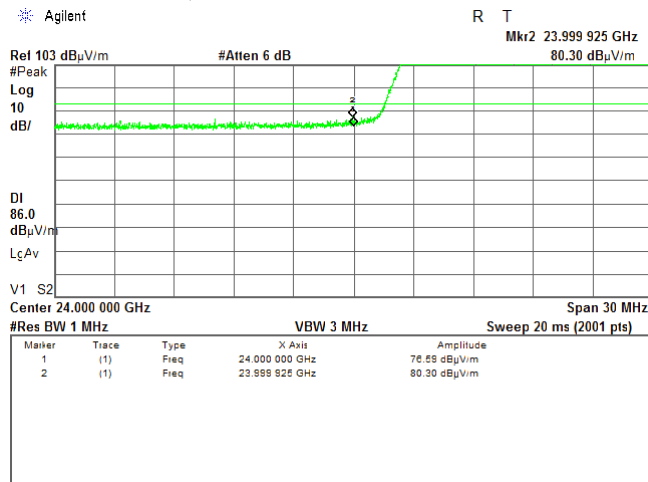
Plot 7.4.6 Low band edge emission test result
