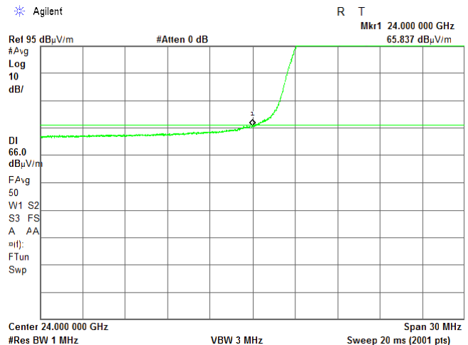
Plot 7.4.14 Low band edge emission test result
