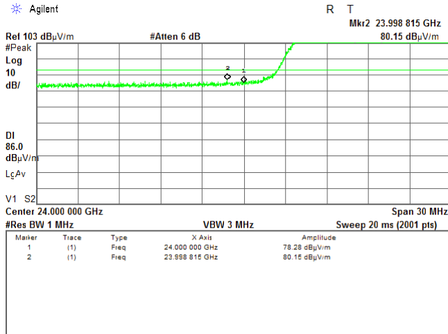
Plot 7.4.22 Low band edge emission test result
