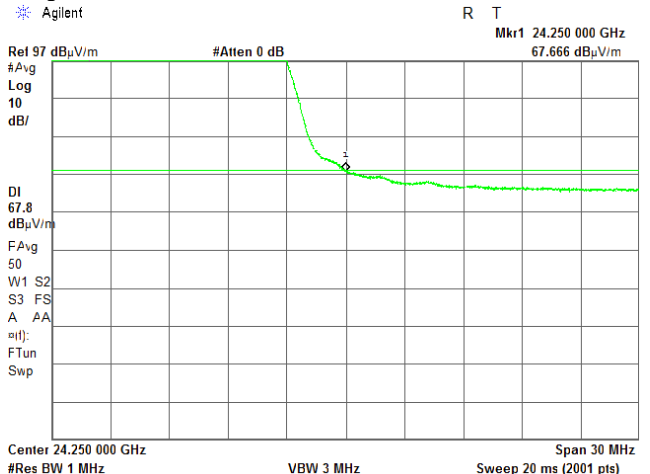
Plot 7.4.12 High band edge emission test result
