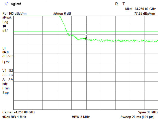
Plot 7.5.36 High band edge emission test result
