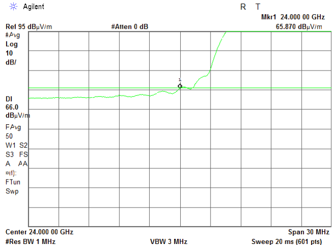
Plot 7.5.30 Low band edge emission test result
