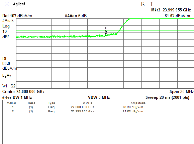
Plot 7.4.38 Low band edge emission test result
