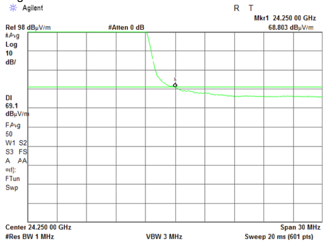
Plot 7.5.4 High band edge emission test result
