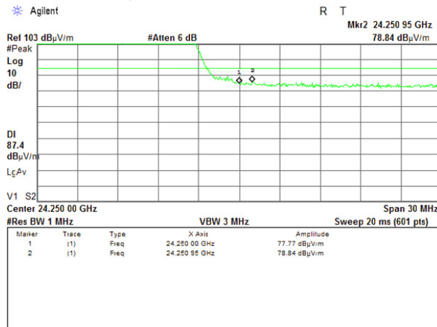
Plot 7.5.12 High band edge emission test result
