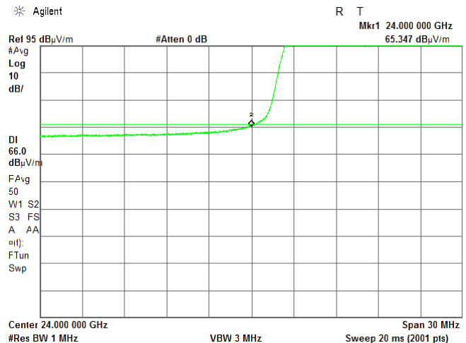
Plot 7.4.6 Low band edge emission test result
