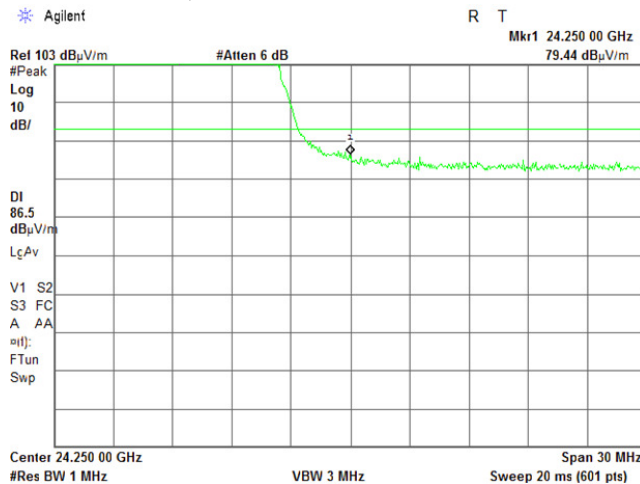
Plot 7.5.20 High band edge emission test result
