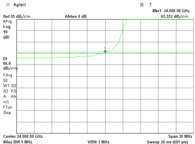
Plot 7.5.22 Low band edge emission test result
