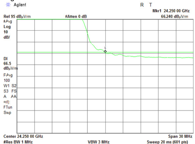
Plot 7.5.20 High band edge emission test result
