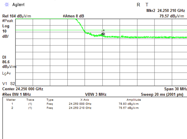
Plot 7.4.28 High band edge emission test result
