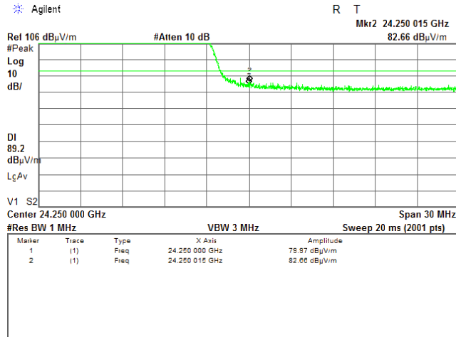
Plot 7.4.4 High band edge emission test result
