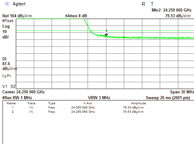
Plot 7.4.20 High band edge emission test result
