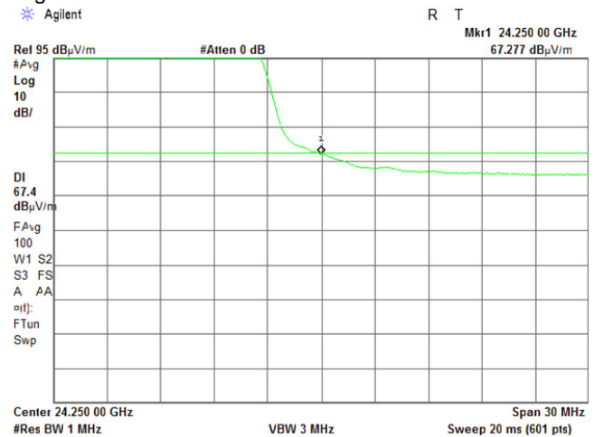
Plot 7.5.12 High band edge emission test result
