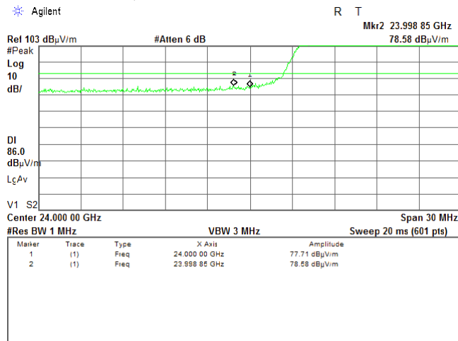
Plot 7.5.22 Low band edge emission test result
