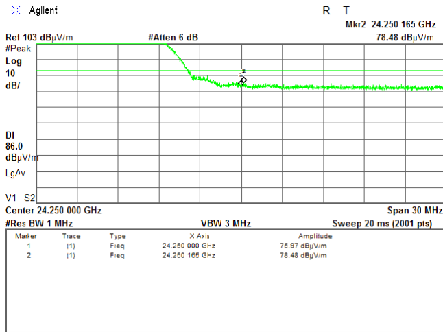
Plot 7.4.40 High band edge emission test result
