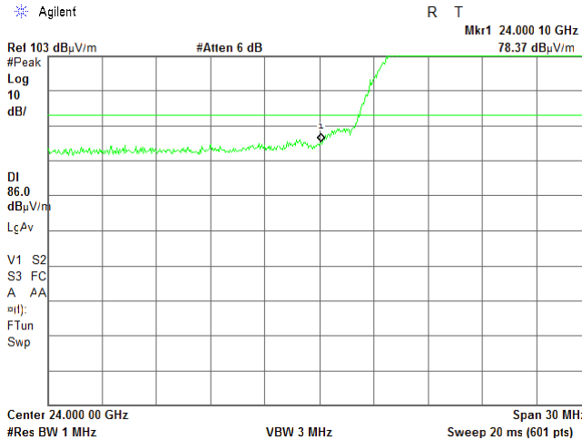
Plot 7.5.38 Low band edge emission test result
