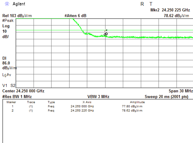
Plot 7.4.36 High band edge emission test result
