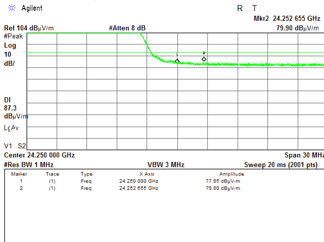
Plot 7.4.24 High band edge emission test result
