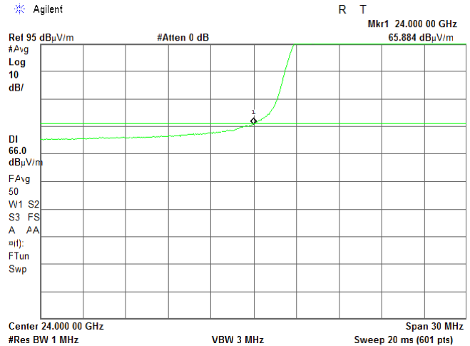
Plot 7.5.14 Low band edge emission test result
