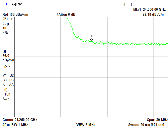
Plot 7.5.28 High band edge emission test result
