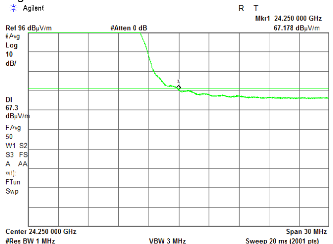
Plot 7.4.24 High band edge emission test result
