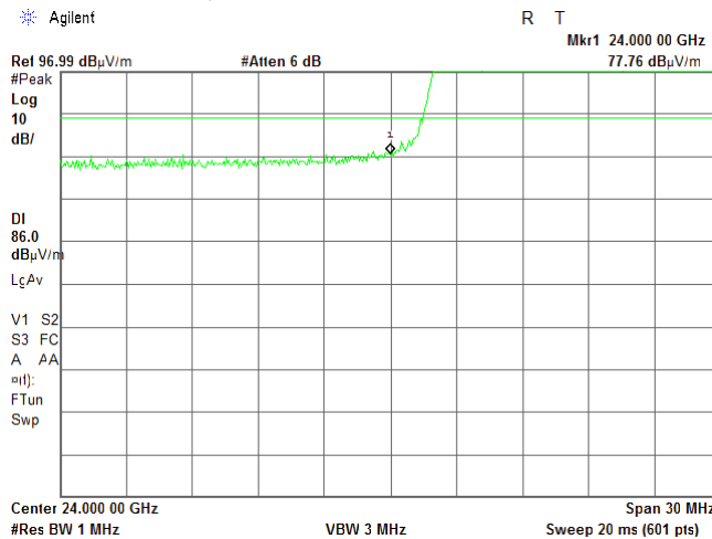
Plot 7.5.6 Low band edge emission test result
