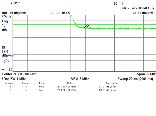
Plot 7.4.12 High band edge emission test result
