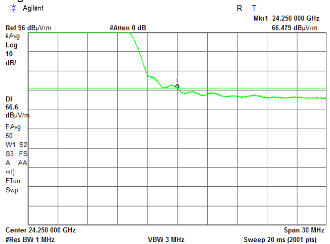
Plot 7.4.28 High band edge emission test result
