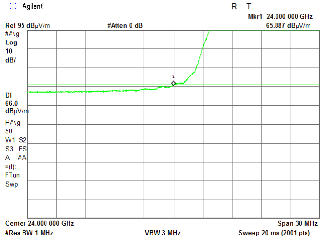
Plot 7.4.22 Low band edge emission test result
