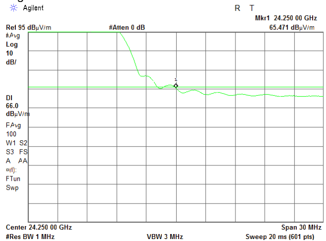
Plot 7.5.36 High band edge emission test result
