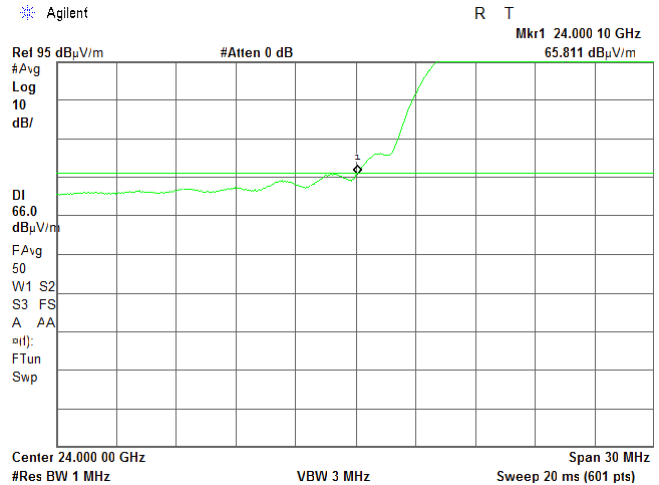
Plot 7.5.38 Low band edge emission test result
