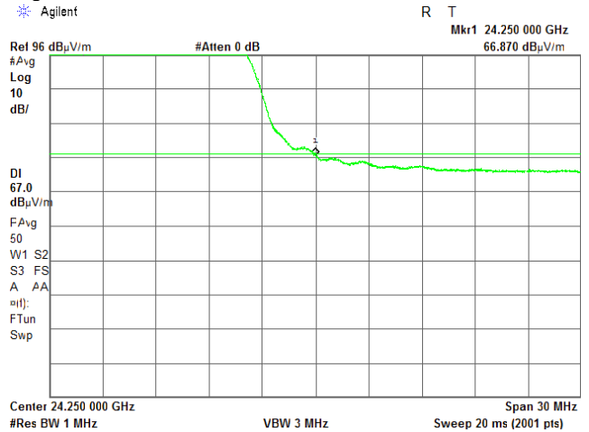
Plot 7.4.20 High band edge emission test result
