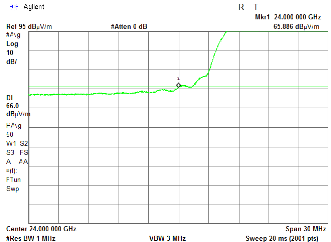
Plot 7.4.26 Low band edge emission test result
