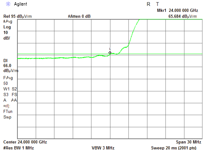
Plot 7.4.30 Low band edge emission test result
