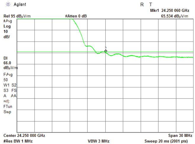
Plot 7.4.40 High band edge emission test result
