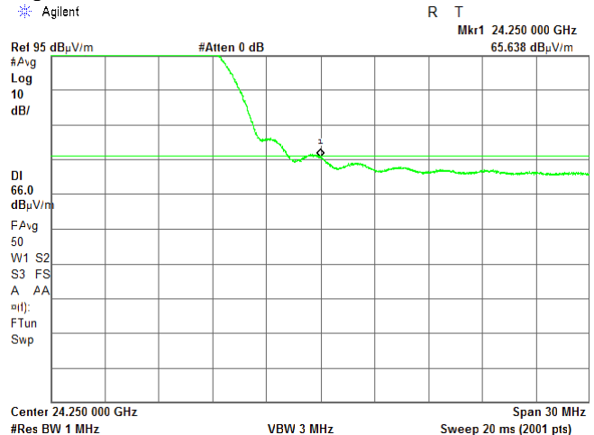
Plot 7.4.36 High band edge emission test result
