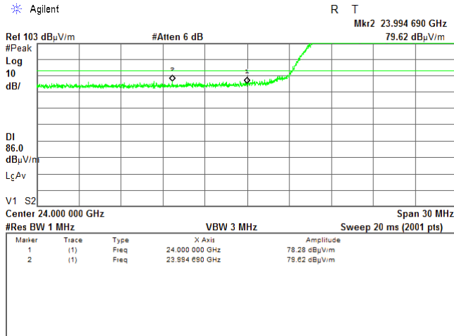
Plot 7.4.26 Low band edge emission test result
