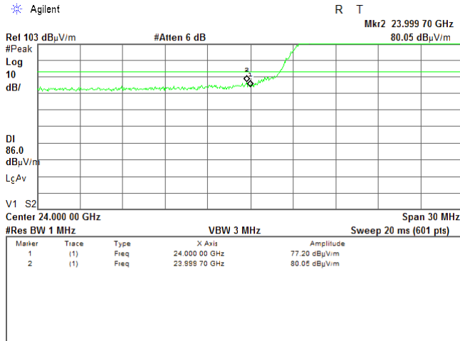
Plot 7.5.30 Low band edge emission test result
