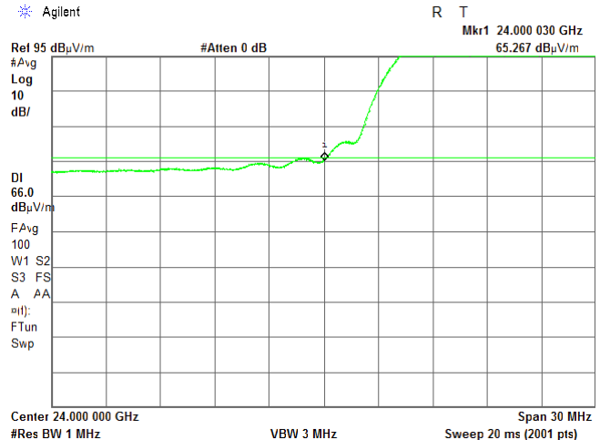
Plot 7.4.38 Low band edge emission test result
