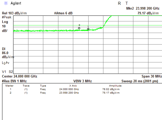
Plot 7.4.30 Low band edge emission test result
