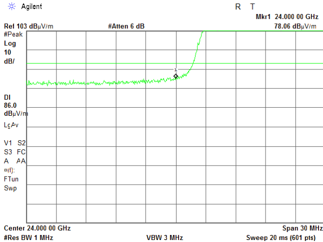
Plot 7.5.14 Low band edge emission test result
