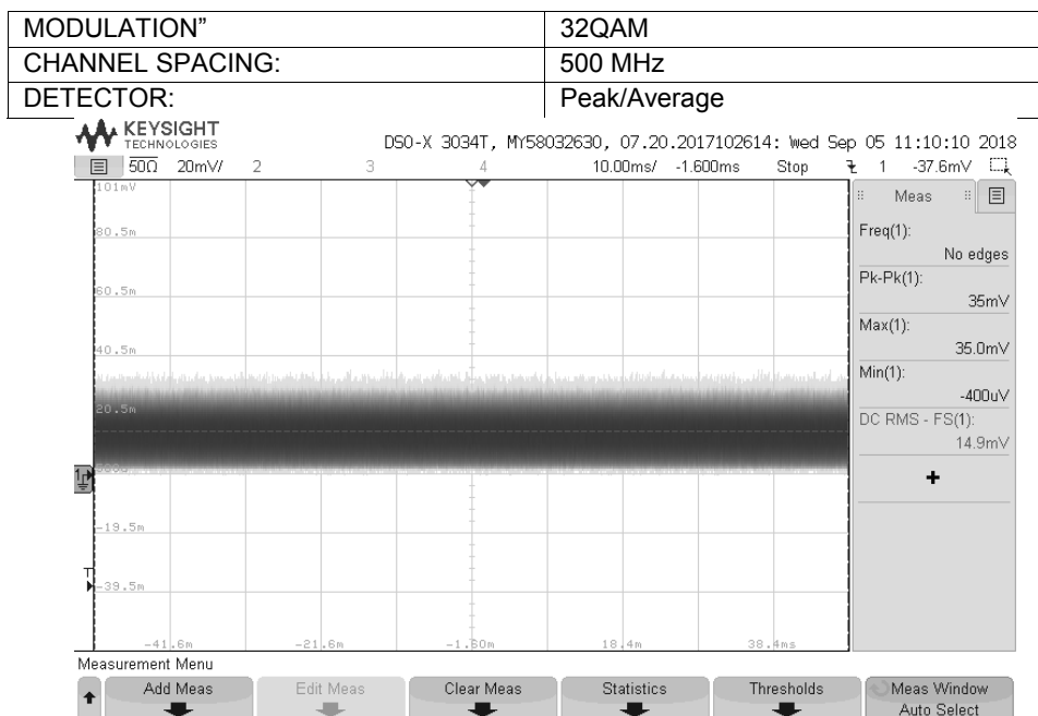
Plot 7.1.84 Output power test result at the high frequency
