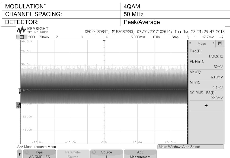
Plot 7.1.5 Output power test result at the mid frequency
