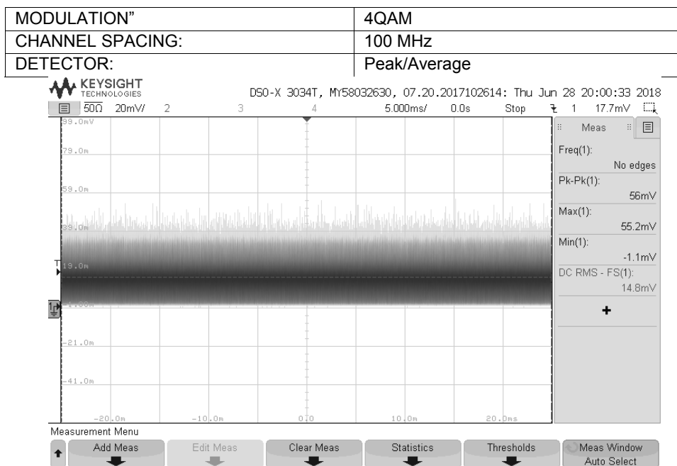
Plot 7.1.26 Output power test result at the mid frequency
