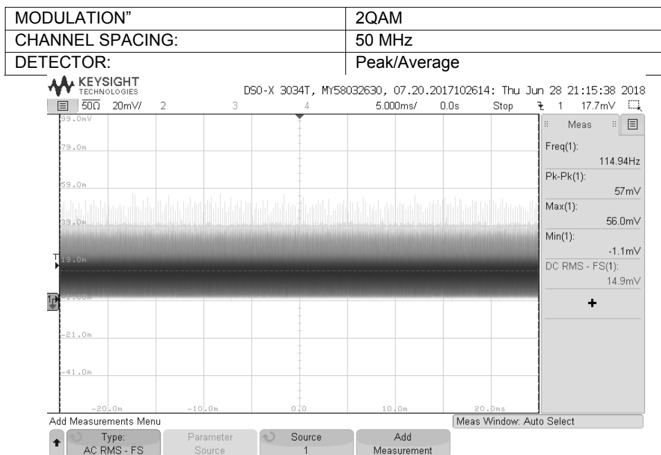
Plot 7.1.1 Output power test result at the low frequency
