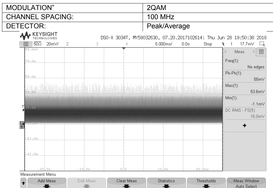
Plot 7.1.23 Output power test result at the mid frequency
