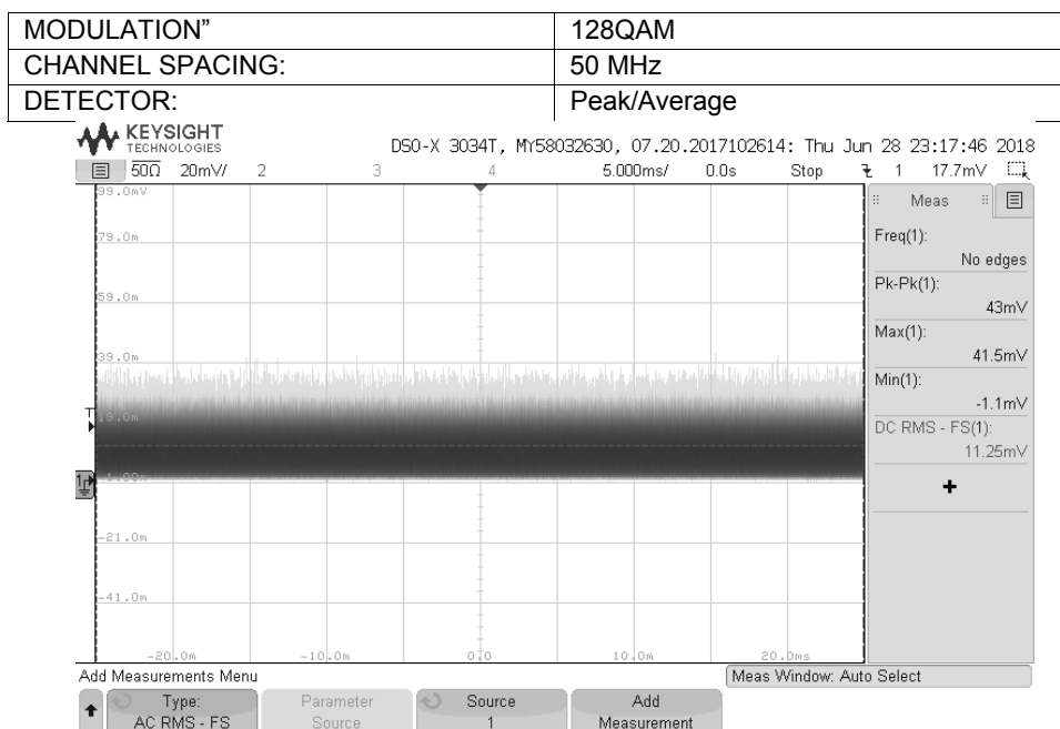
Plot 7.1.20 Output power test result at the mid frequency
