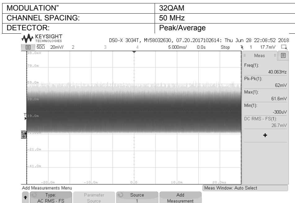
Plot 7.1.15 Output power test result at the high frequency
