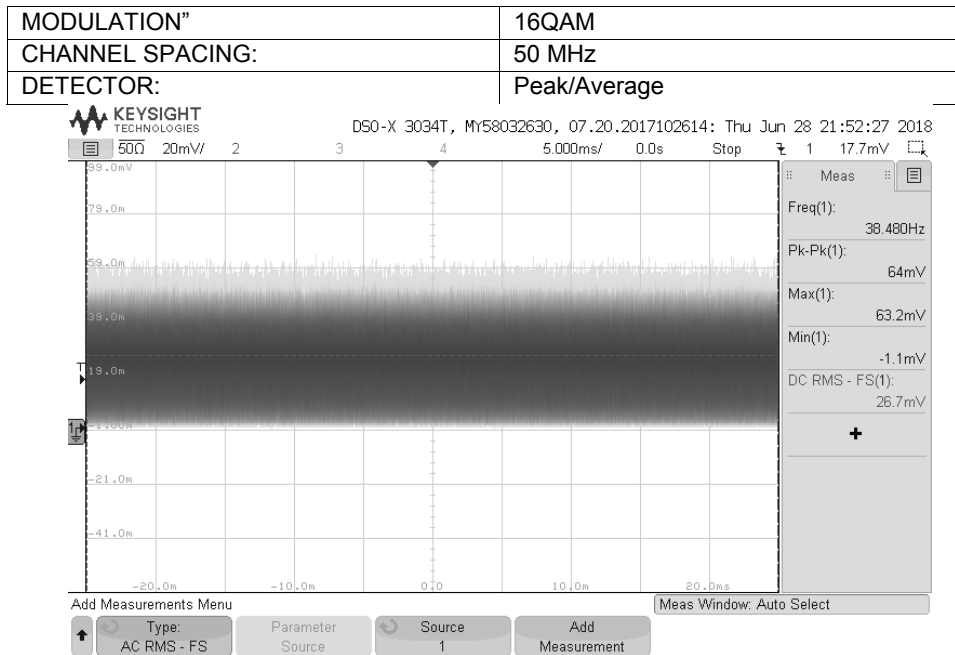
Plot 7.1.12 Output power test result at the high frequency
