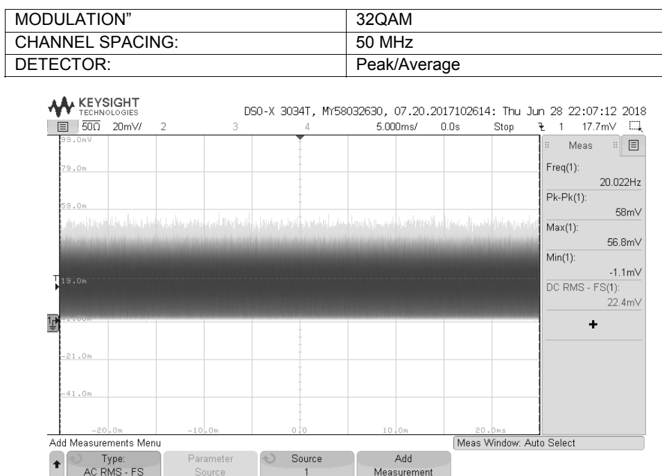
Plot 7.1.14 Output power test result at the mid frequency
