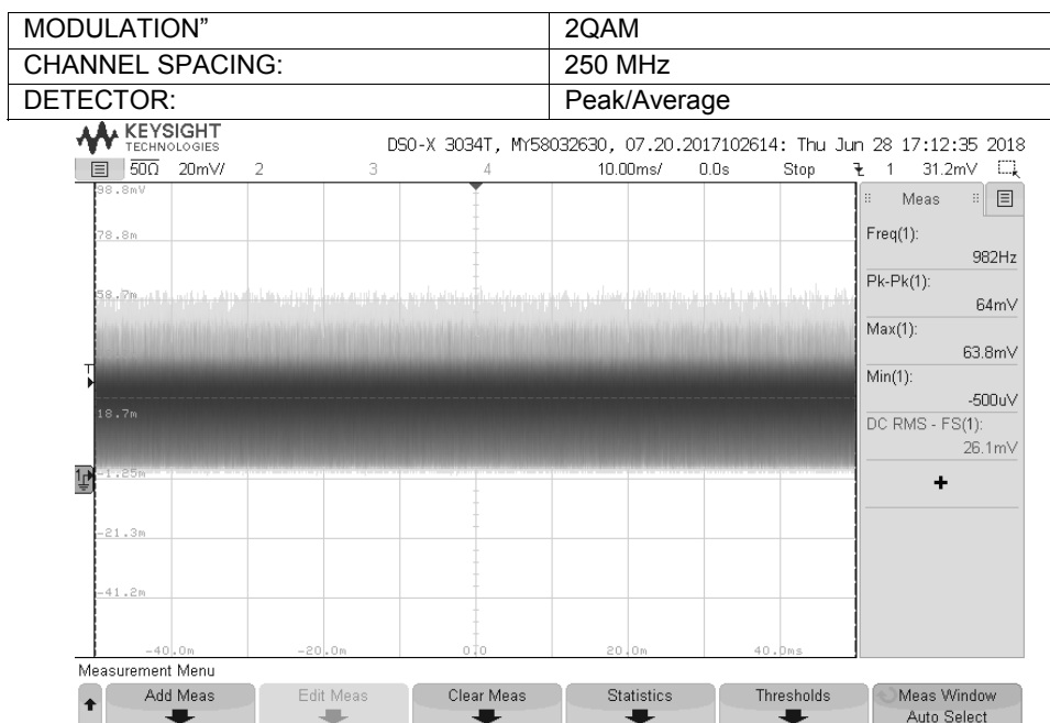
Plot 7.1.47 Output power test result at the mid frequency
