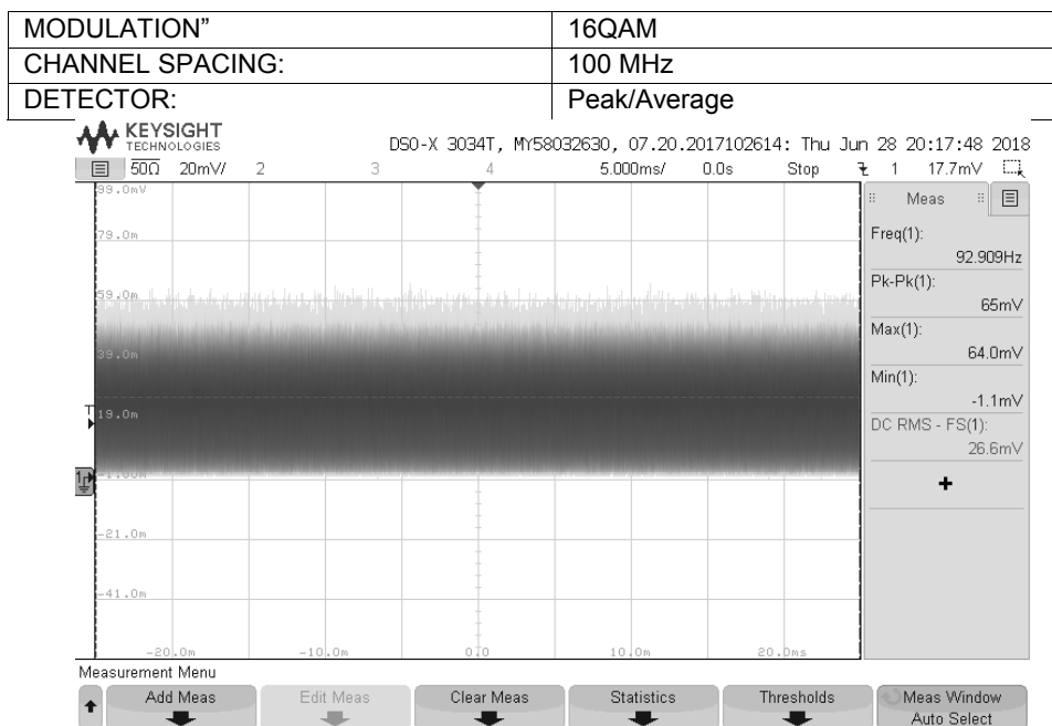
Plot 7.1.33 Output power test result at the high frequency
