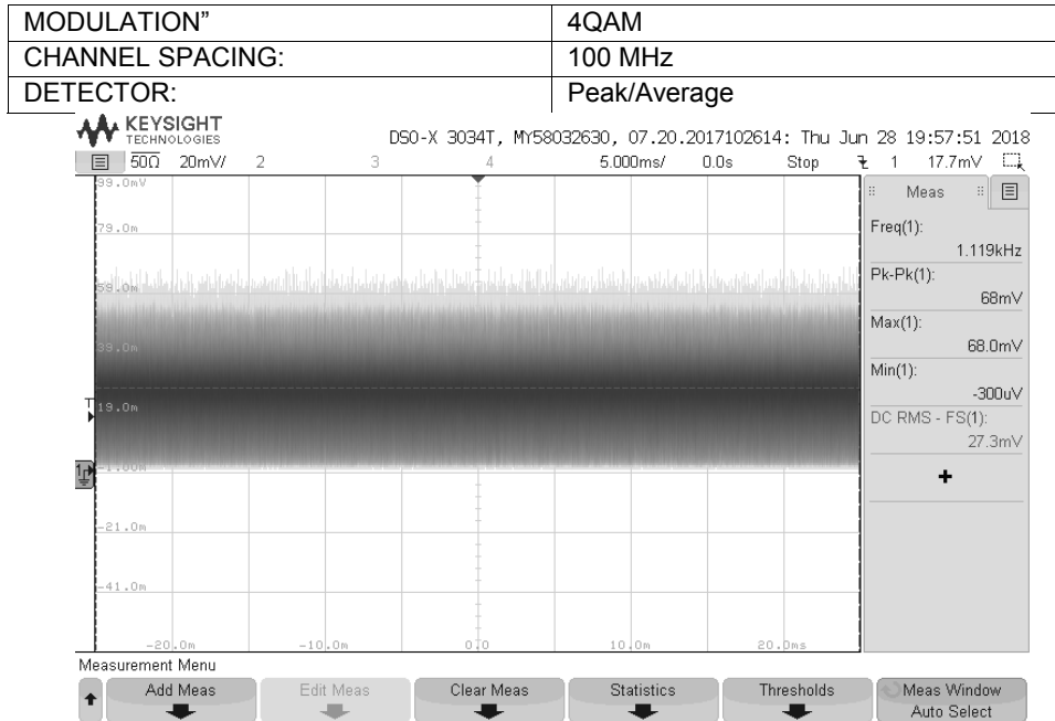
Plot 7.1.27 Output power test result at the high frequency
