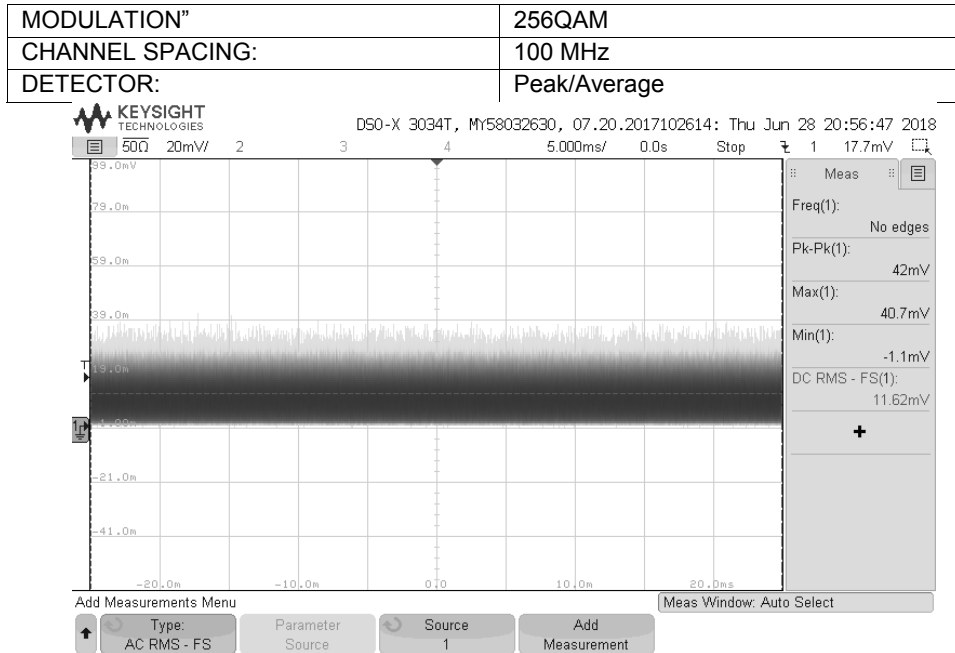
Plot 7.1.45 Output power test result at the high frequency
