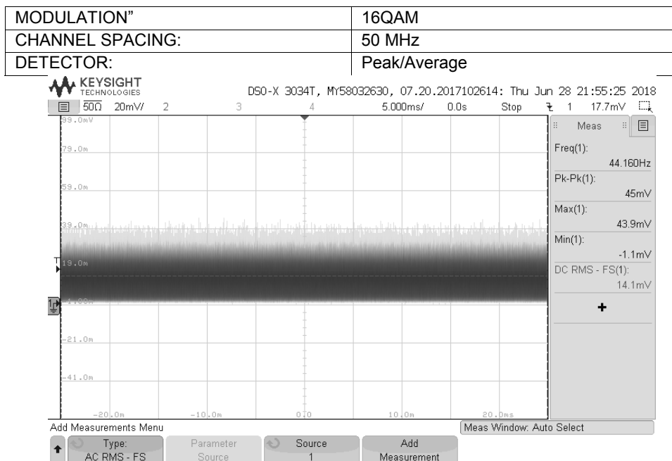
Plot 7.1.11 Output power test result at the mid frequency
