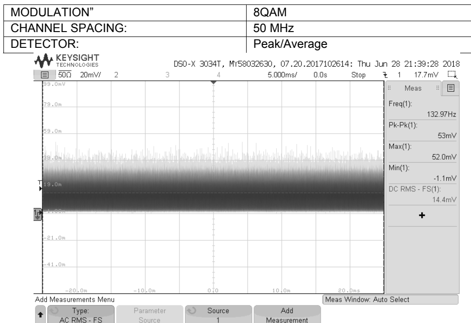
Plot 7.1.8 Output power test result at the mid frequency
