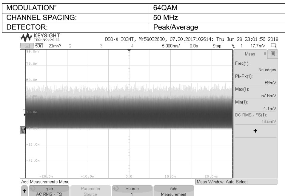
Plot 7.1.17 Output power test result at the mid frequency
