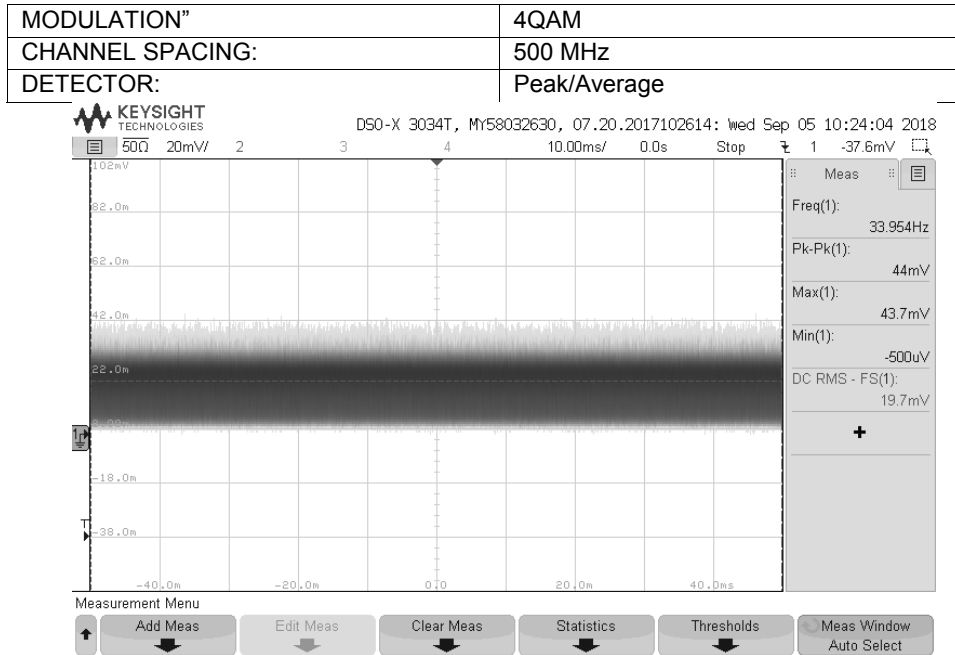
Plot 7.1.75 Output power test result at the high frequency
