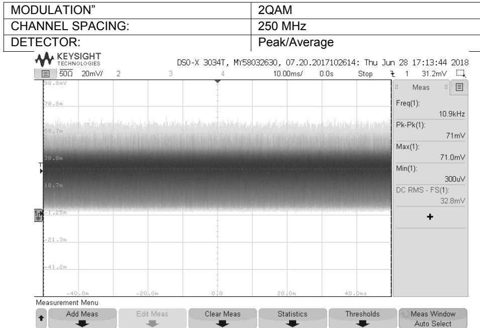
Plot 7.1.48 Output power test result at the high frequency
