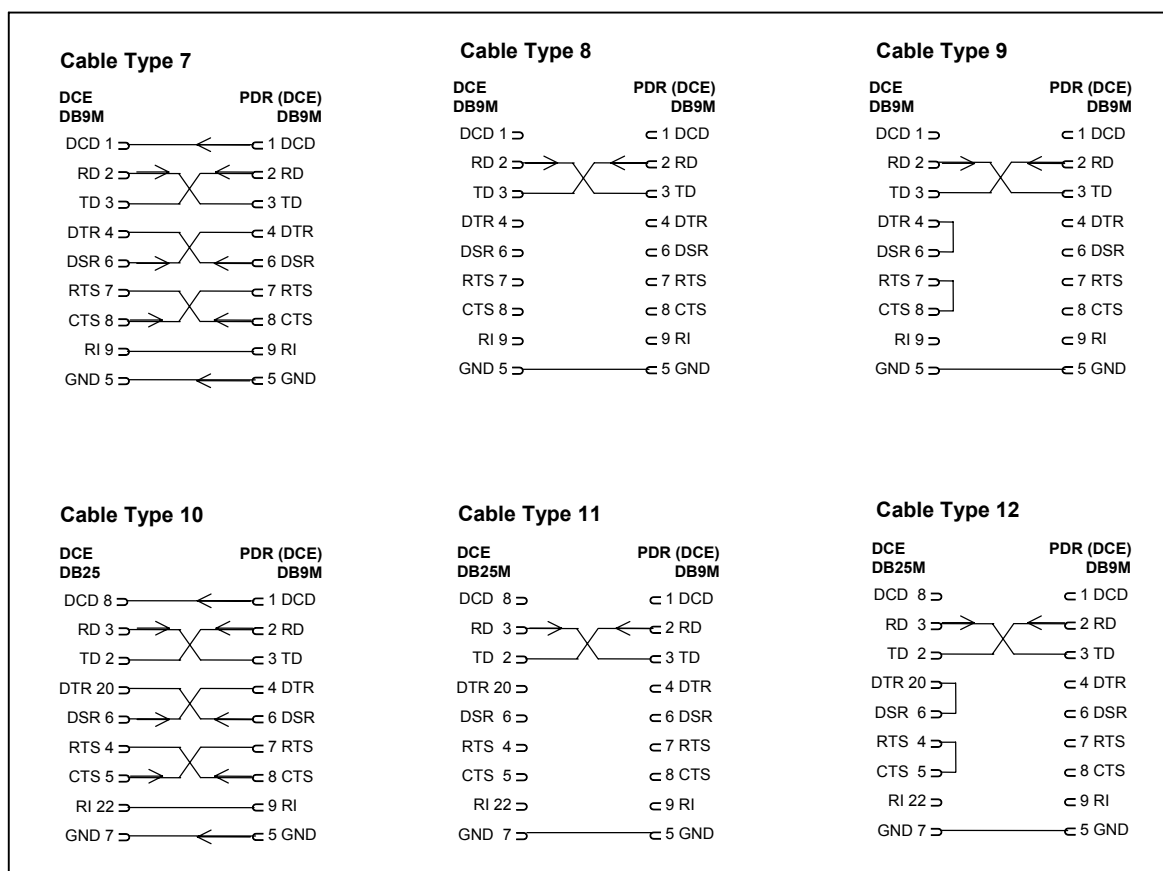
Figure 5. DCE-DCE serial cable configurations
