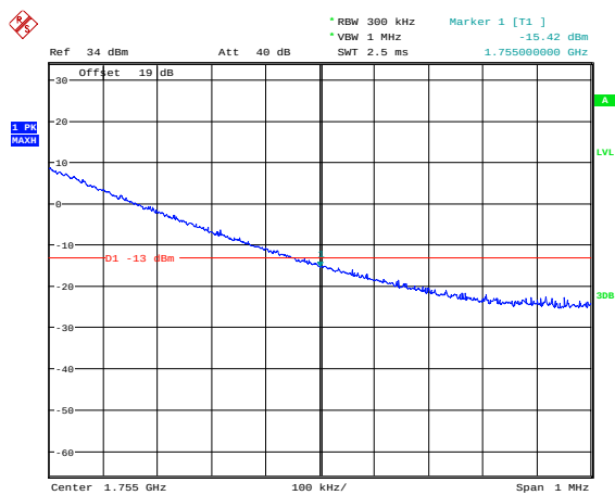
Highest Channel / 15MHz / QPSK / 1RB
