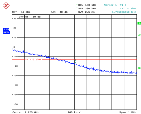
Highest Channel / 15MHz / QPSK / Full RB
