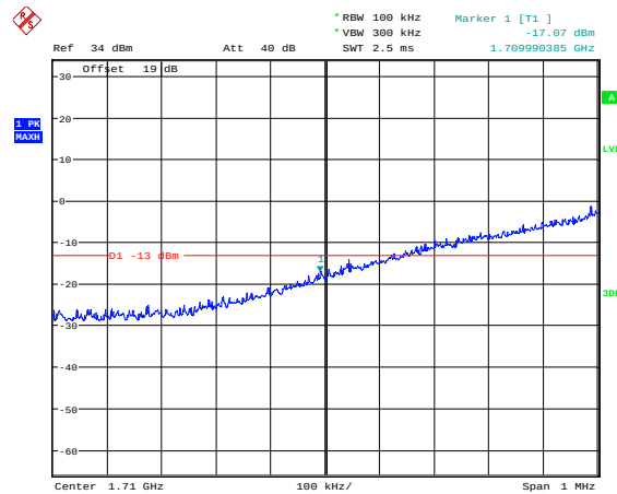
Lowest Channel / 15MHz / QPSK / Full RB
