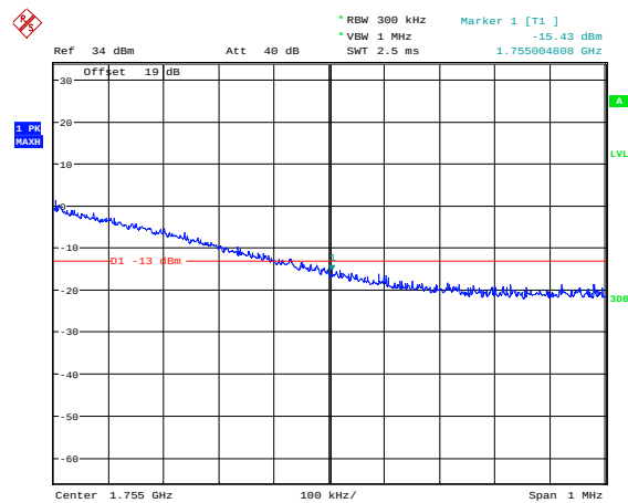
Highest Channel / 20MHz / 16QAM / Full RB
