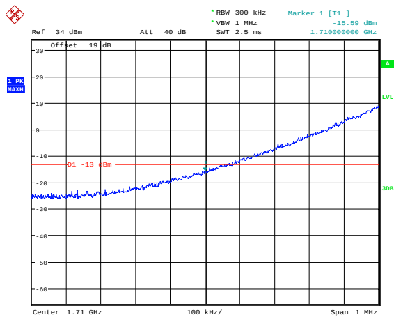
Lowest Channel / 15MHz / 16QAM / 1RB
