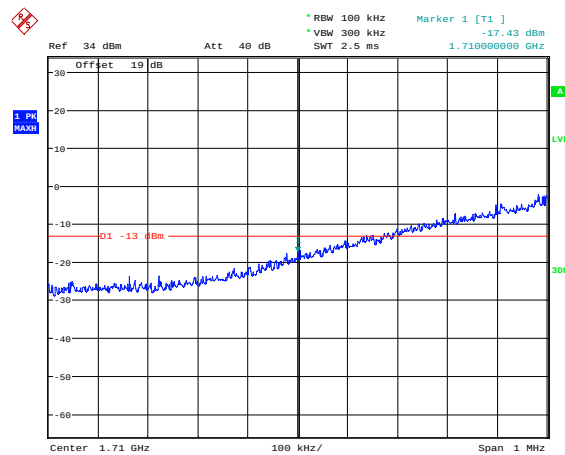
Lowest Channel / 15MHz / 16QAM / Full RB
