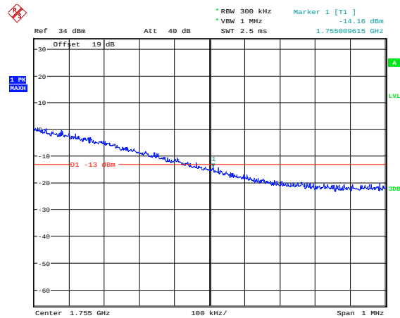
Highest Channel / 20MHz / QPSK / Full RB
