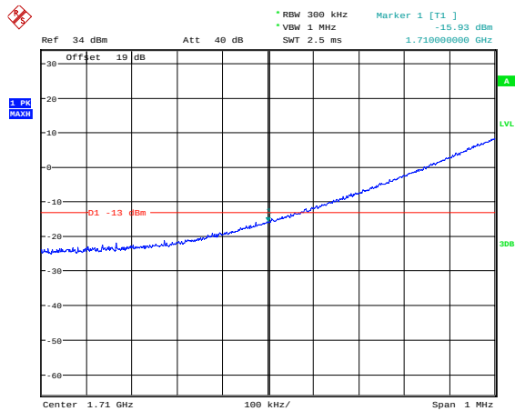
Lowest Channel / 15MHz / QPSK / 1RB
