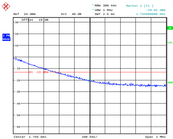
Highest Channel / 20MHz / 16QAM / 1RB
