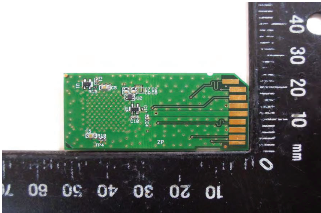
Back View of EUT
