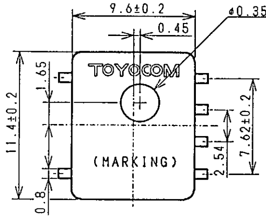
PIN CONNECTION(TOP VIEW)
