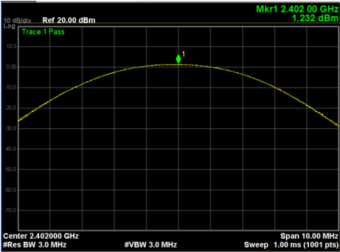
Bluetooth 8-DPSK Channel 0
