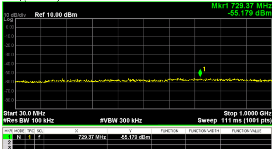
Channel 39; (30~1000) MHz
