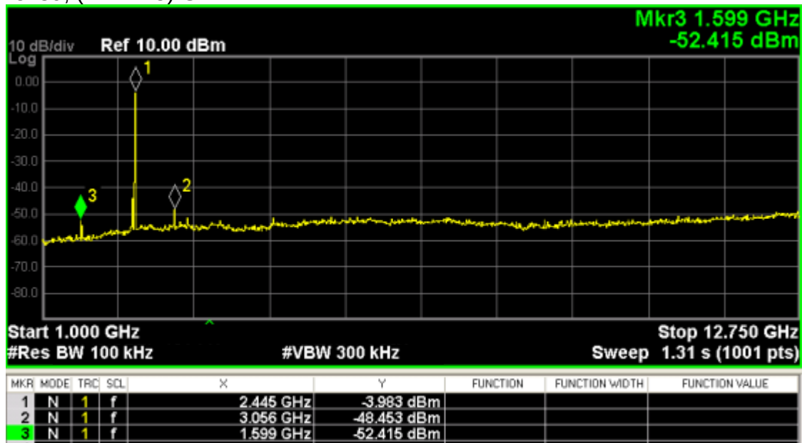
Channel 39; (1~12.75) GHz
