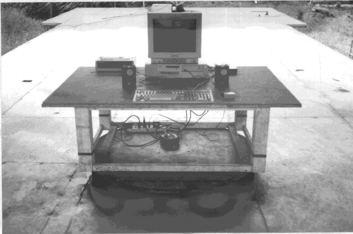
(Front View)
