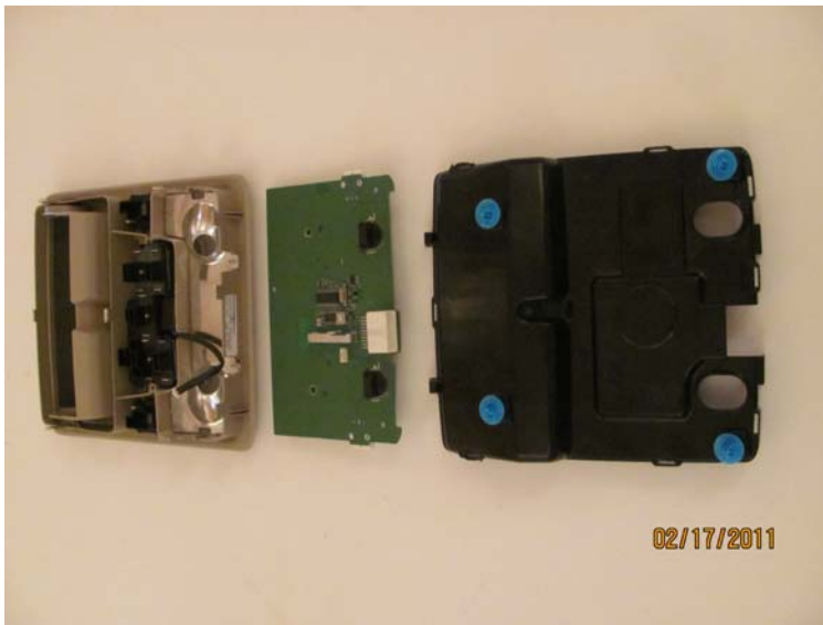
Rear View with HL apart from Assembly Unit
