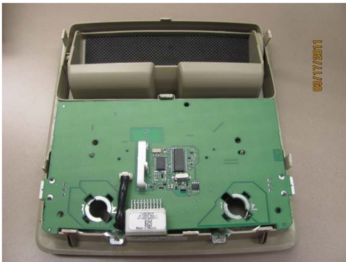
Rear View without back housing
