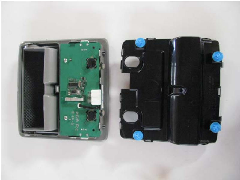
Rear View with HL in Assembly Unit
