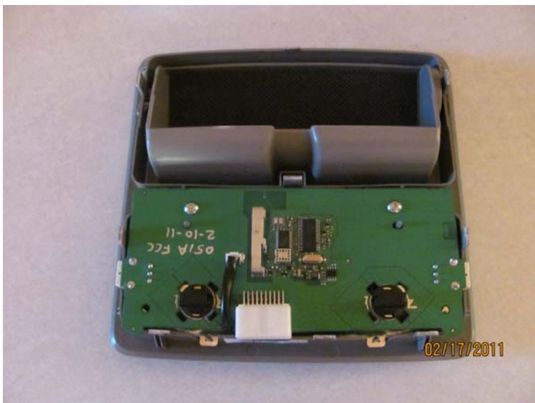
Rear View without back housing
